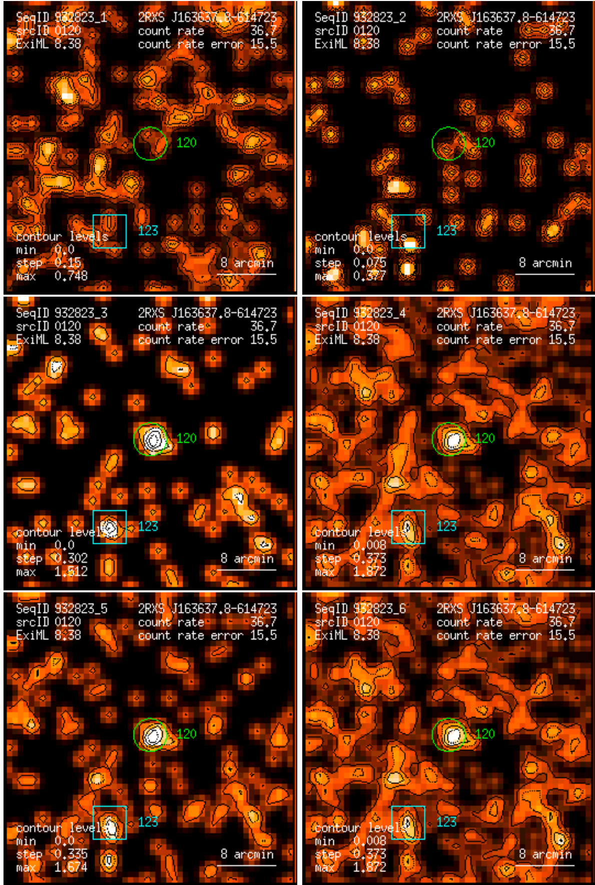
Figure 120: RASS 932823: detection 0120: band rate images, Gaussian filter: (1) PSPC channels 11 – 41, (2) 52 – 90, (3) 91 – 201, (4) 11 – 235, (5) 52 – 201, (6) 11 – 201. Broad band rates in counts/ks. Band rate contour levels in counts/ks/arcmin 2 .
