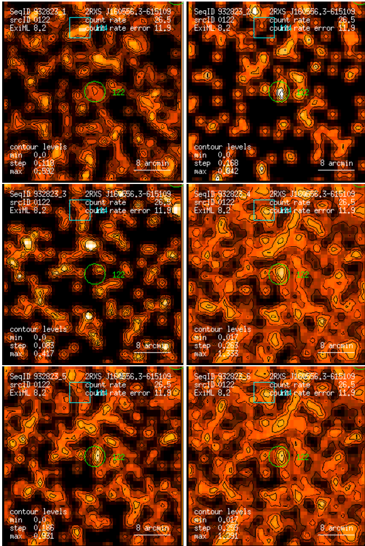
Figure 122: RASS 932823: detection 0122: band rate images, Gaussian filter: (1) PSPC channels 11 – 41, (2) 52 – 90, (3) 91 – 201, (4) 11 – 235, (5) 52 – 201, (6) 11 – 201. Broad band rates in counts/ks. Band rate contour levels in counts/ks/arcmin 2 .
