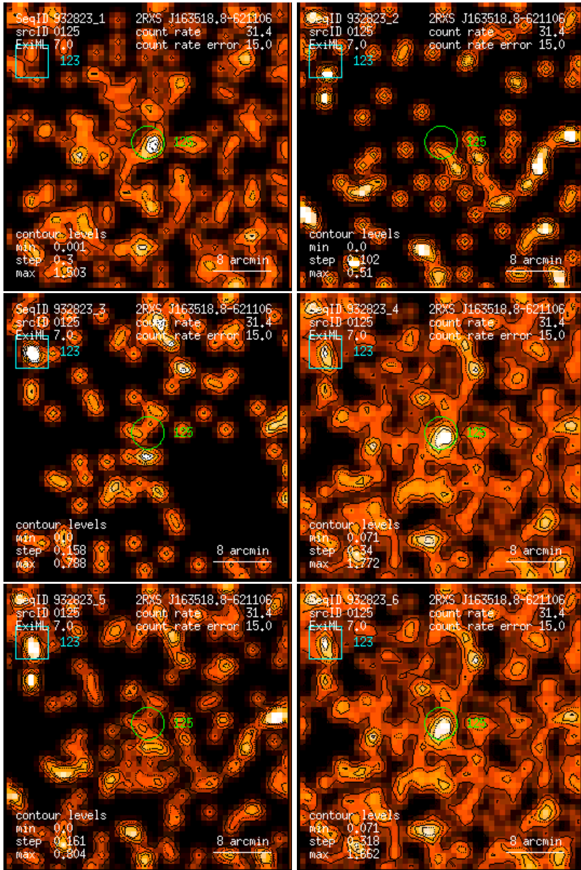
Figure 125: RASS 932823: detection 0125: band rate images, Gaussian filter: (1) PSPC channels 11 – 41, (2) 52 – 90, (3) 91 – 201, (4) 11 – 235, (5) 52 – 201, (6) 11 – 201. Broad band rates in counts/ks. Band rate contour levels in counts/ks/arcmin 2 .
