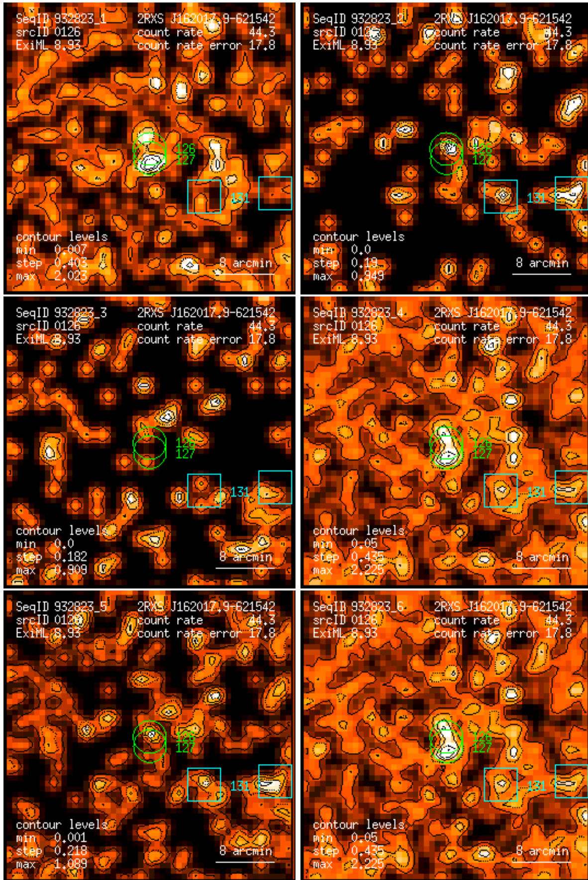
Figure 126: RASS 932823: detection 0126: band rate images, Gaussian filter: (1) PSPC channels 11 – 41, (2) 52 – 90, (3) 91 – 201, (4) 11 – 235, (5) 52 – 201, (6) 11 – 201. Broad band rates in counts/ks. Band rate contour levels in counts/ks/arcmin 2 .
