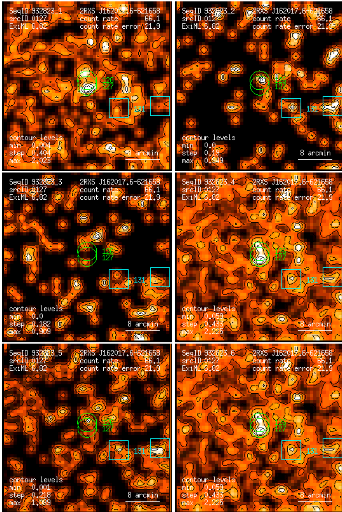
Figure 127: RASS 932823: detection 0127: band rate images, Gaussian filter: (1) PSPC channels 11 – 41, (2) 52 – 90, (3) 91 – 201, (4) 11 – 235, (5) 52 – 201, (6) 11 – 201. Broad band rates in counts/ks. Band rate contour levels in counts/ks/arcmin 2 .
