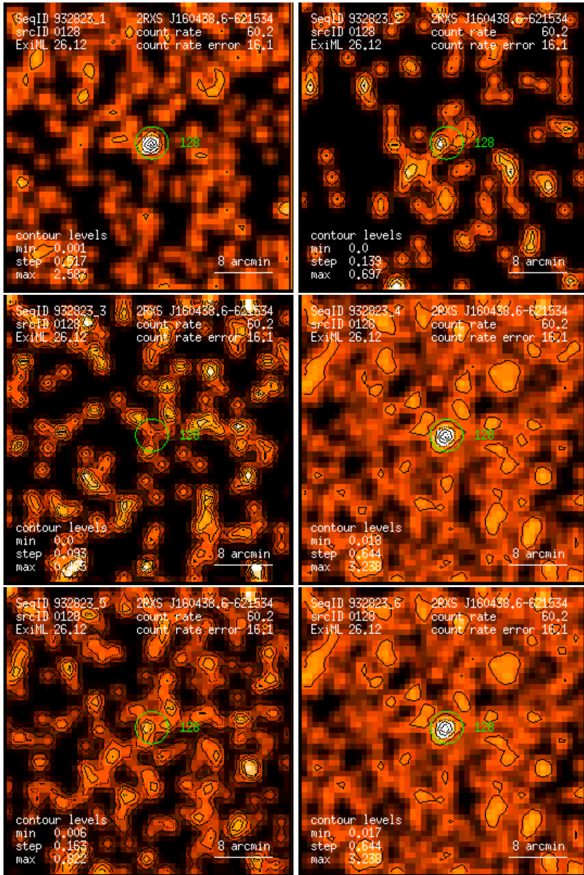
Figure 128: RASS 932823: detection 0128: band rate images, Gaussian filter: (1) PSPC channels 11 – 41, (2) 52 – 90, (3) 91 – 201, (4) 11 – 235, (5) 52 – 201, (6) 11 – 201. Broad band rates in counts/ks. Band rate contour levels in counts/ks/arcmin 2 .
