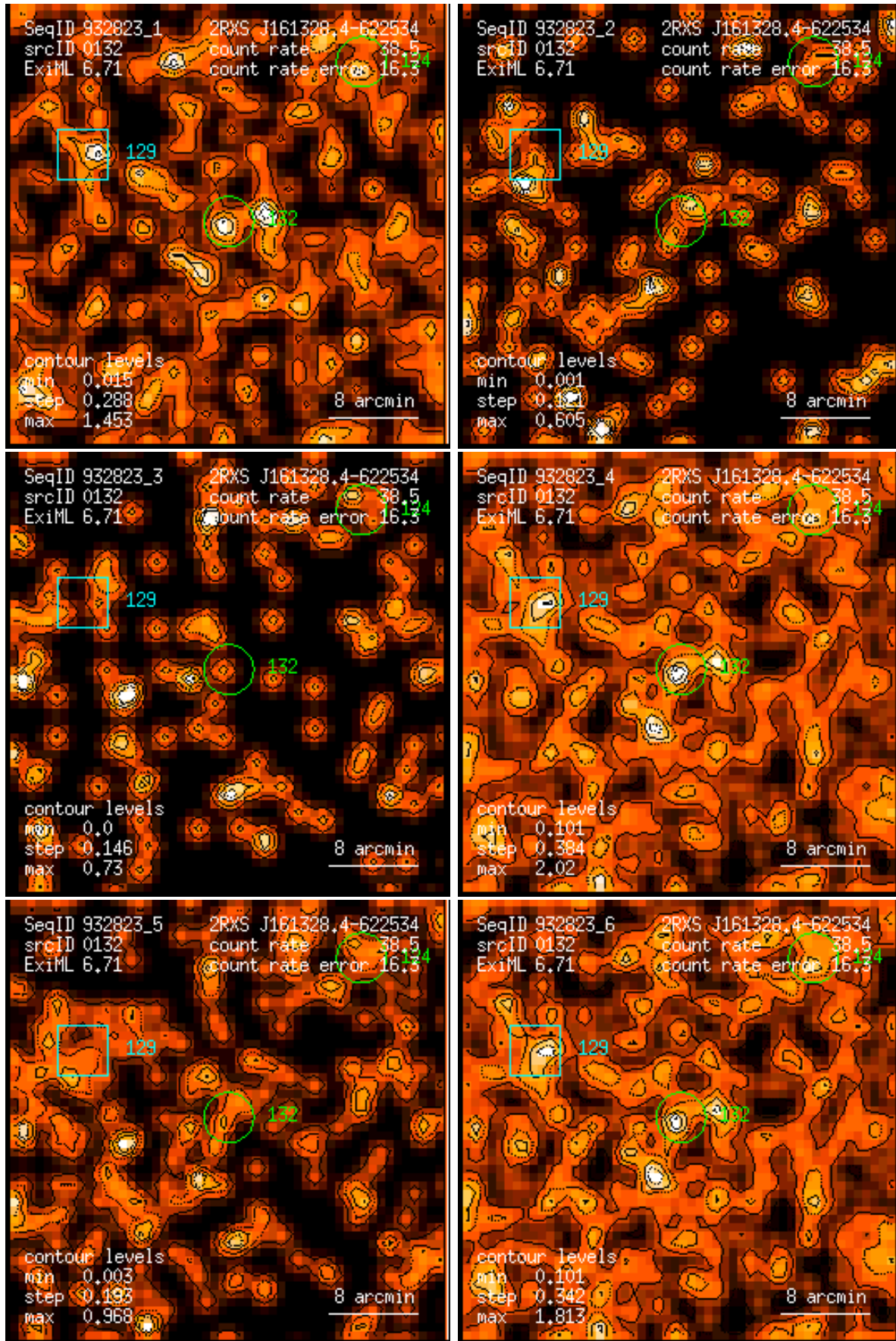
Figure 132: RASS 932823: detection 0132: band rate images, Gaussian filter: (1) PSPC channels 11 – 41, (2) 52 – 90, (3) 91 – 201, (4) 11 – 235, (5) 52 – 201, (6) 11 – 201. Broad band rates in counts/ks. Band rate contour levels in counts/ks/arcmin 2 .
