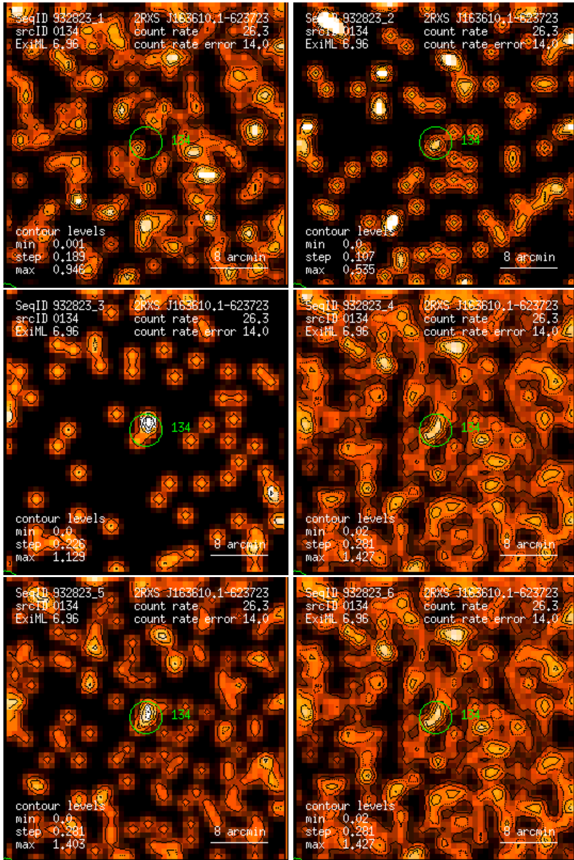
Figure 134: RASS 932823: detection 0134: band rate images, Gaussian filter: (1) PSPC channels 11 – 41, (2) 52 – 90, (3) 91 – 201, (4) 11 – 235, (5) 52 – 201, (6) 11 – 201. Broad band rates in counts/ks. Band rate contour levels in counts/ks/arcmin 2 .
