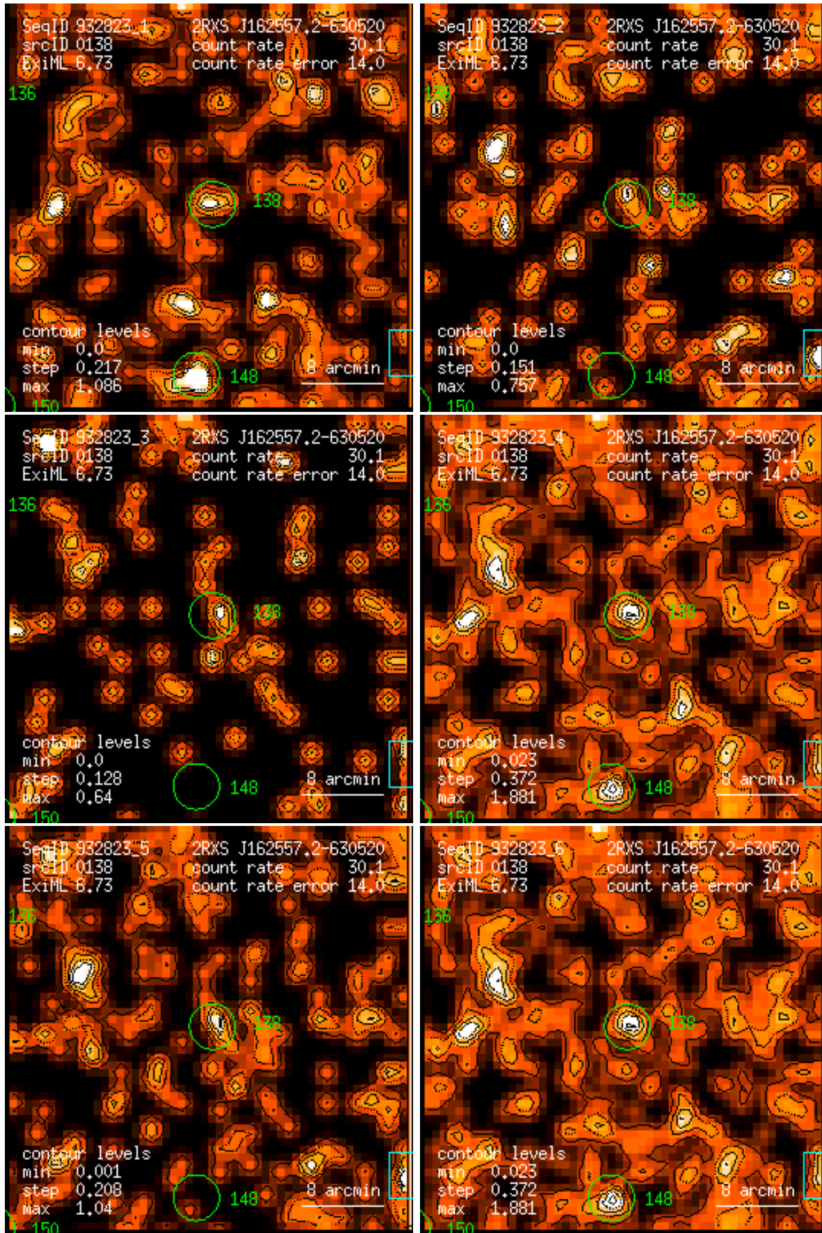
Figure 138: RASS 932823: detection 0138: band rate images, Gaussian filter: (1) PSPC channels 11 – 41, (2) 52 – 90, (3) 91 – 201, (4) 11 – 235, (5) 52 – 201, (6) 11 – 201. Broad band rates in counts/ks. Band rate contour levels in counts/ks/arcmin 2 .
