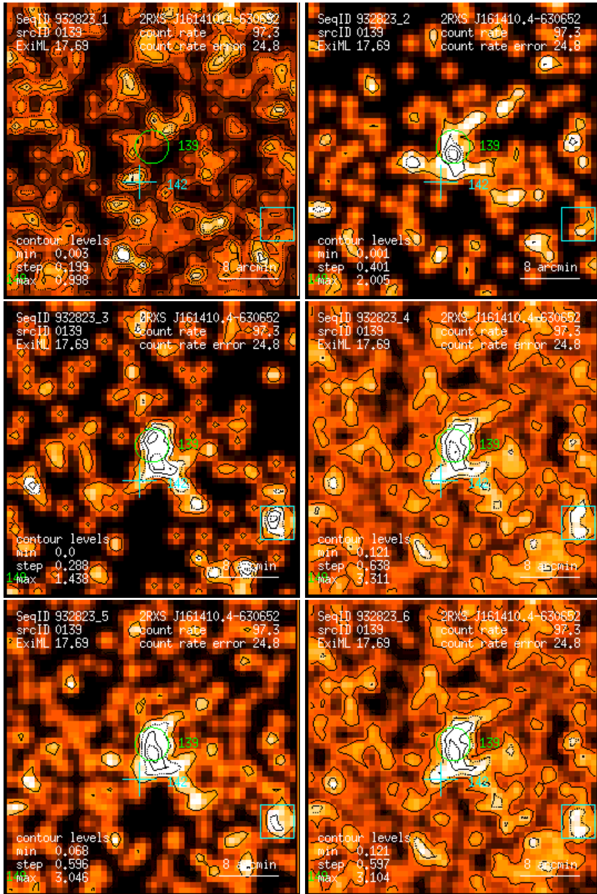
Figure 139: RASS 932823: detection 0139: band rate images, Gaussian filter: (1) PSPC channels 11 – 41, (2) 52 – 90, (3) 91 – 201, (4) 11 – 235, (5) 52 – 201, (6) 11 – 201. Broad band rates in counts/ks. Band rate contour levels in counts/ks/arcmin 2 .
