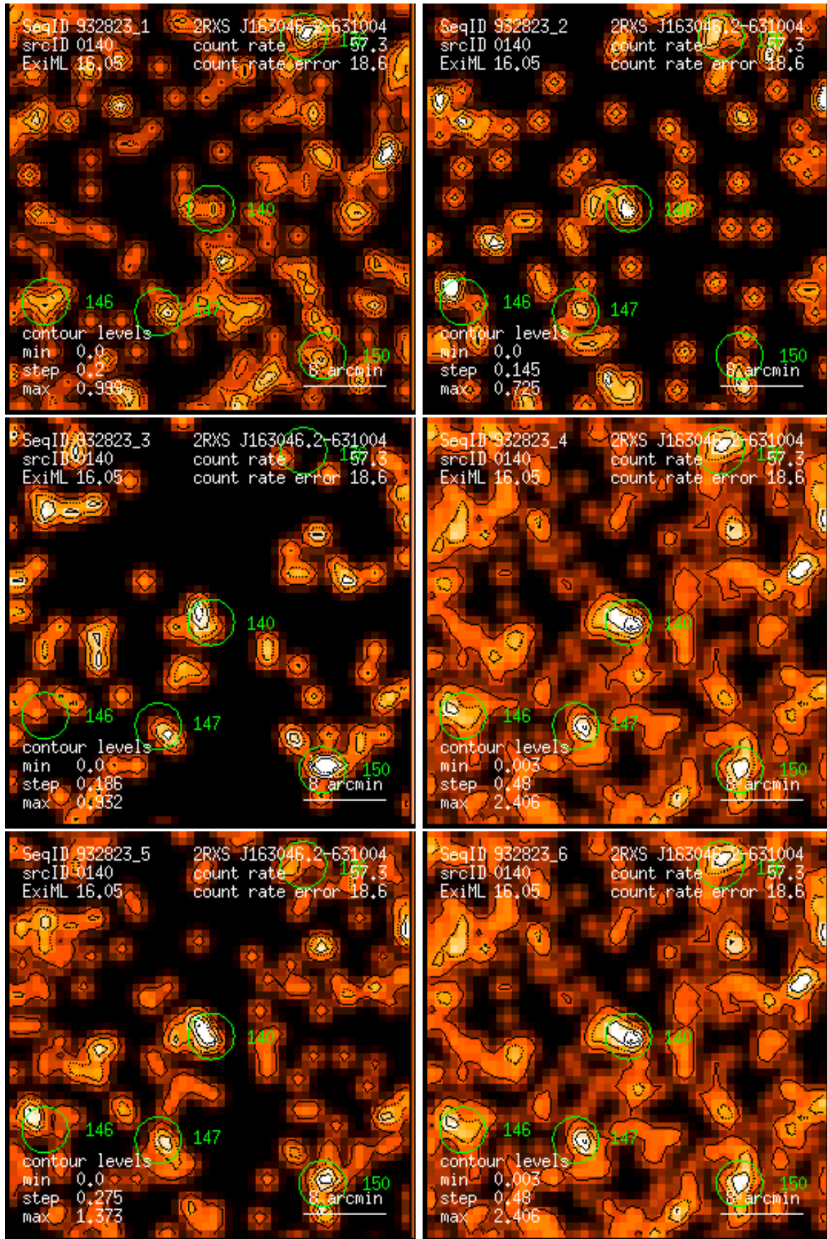
Figure 140: RASS 932823: detection 0140: band rate images, Gaussian filter: (1) PSPC channels 11 – 41, (2) 52 – 90, (3) 91 – 201, (4) 11 – 235, (5) 52 – 201, (6) 11 – 201. Broad band rates in counts/ks. Band rate contour levels in counts/ks/arcmin 2 .
