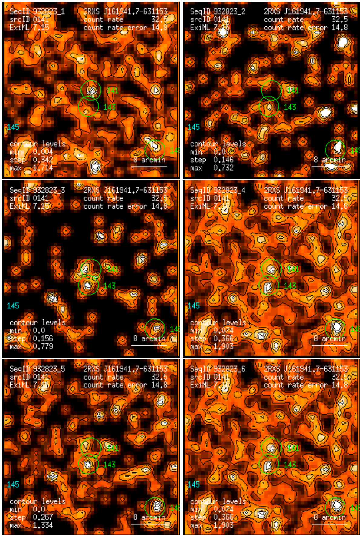
Figure 141: RASS 932823: detection 0141: band rate images, Gaussian filter: (1) PSPC channels 11 – 41, (2) 52 – 90, (3) 91 – 201, (4) 11 – 235, (5) 52 – 201, (6) 11 – 201. Broad band rates in counts/ks. Band rate contour levels in counts/ks/arcmin 2 .
