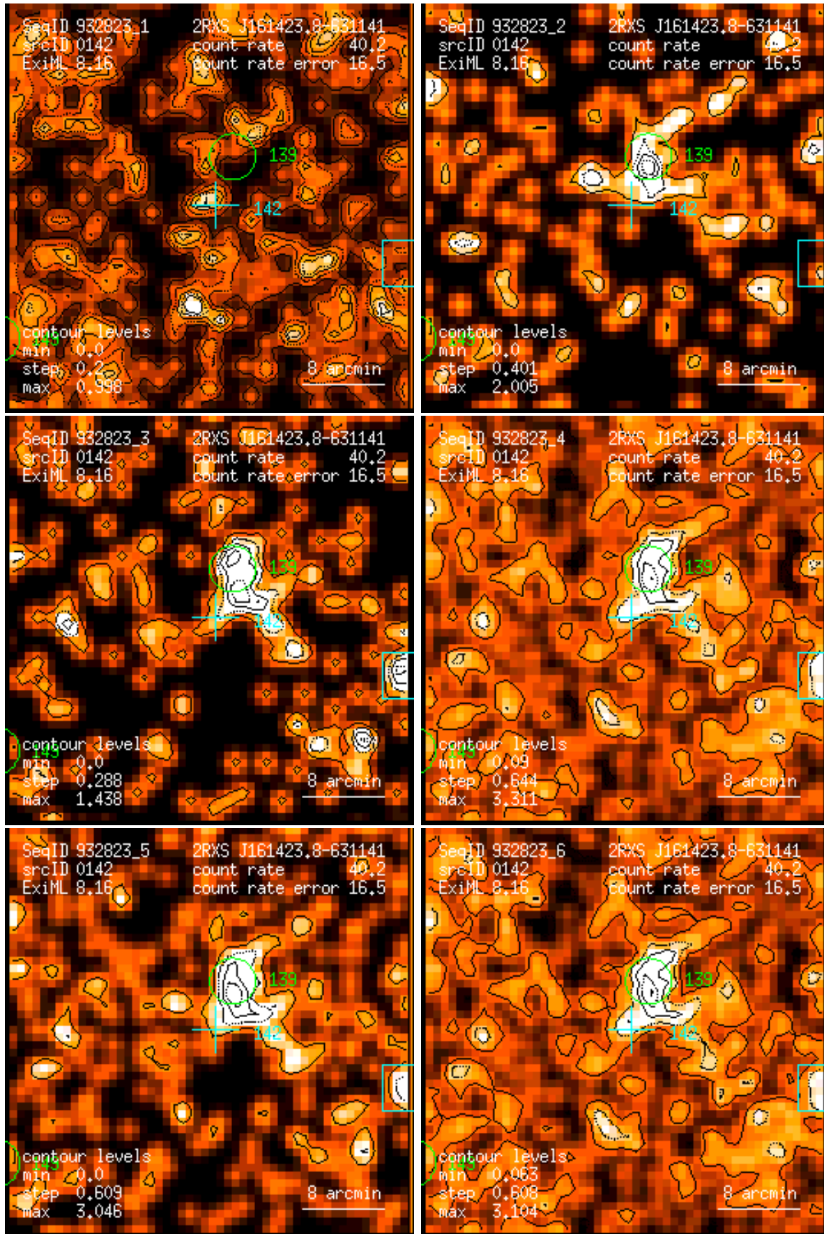
Figure 142: RASS 932823: detection 0142: band rate images, Gaussian filter: (1) PSPC channels 11 – 41, (2) 52 – 90, (3) 91 – 201, (4) 11 – 235, (5) 52 – 201, (6) 11 – 201. Broad band rates in counts/ks. Band rate contour levels in counts/ks/arcmin 2 .
