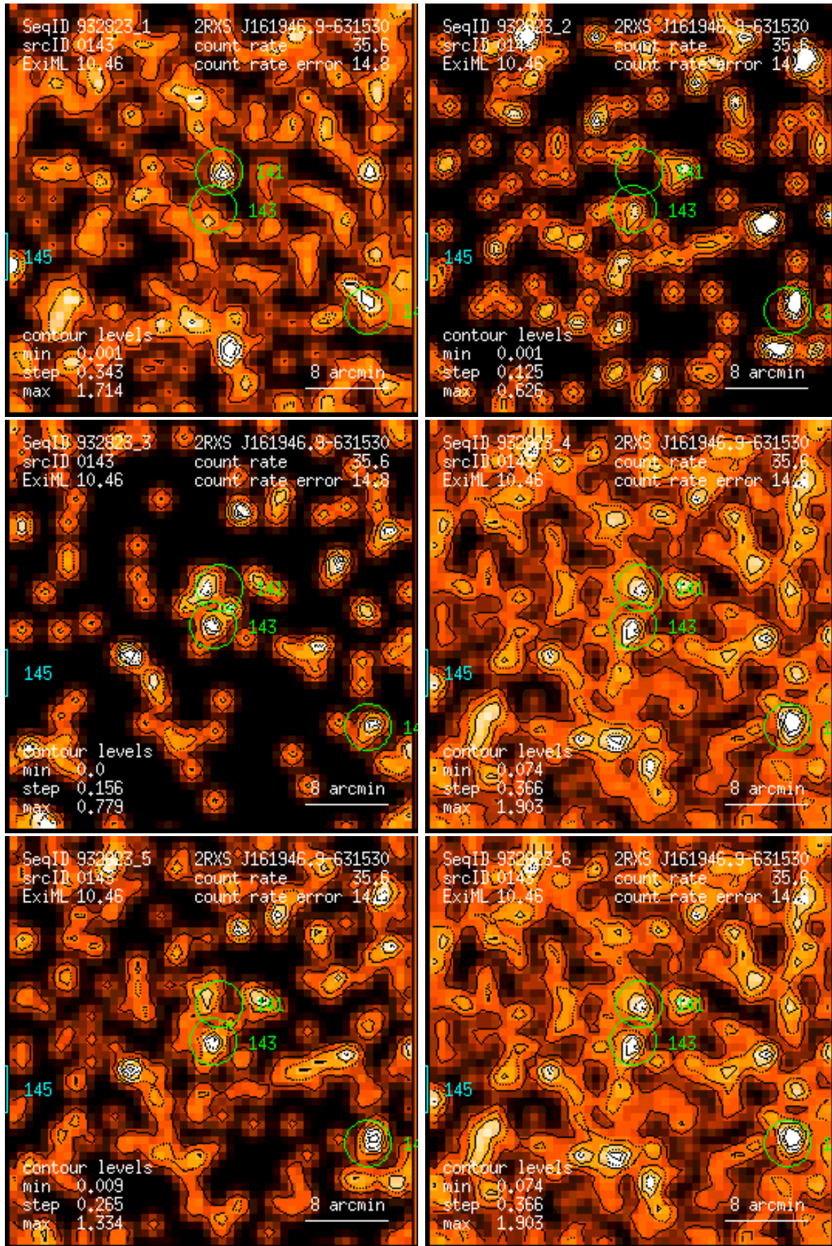
Figure 143: RASS 932823: detection 0143: band rate images, Gaussian filter: (1) PSPC channels 11 – 41, (2) 52 – 90, (3) 91 – 201, (4) 11 – 235, (5) 52 – 201, (6) 11 – 201. Broad band rates in counts/ks. Band rate contour levels in counts/ks/arcmin 2 .
