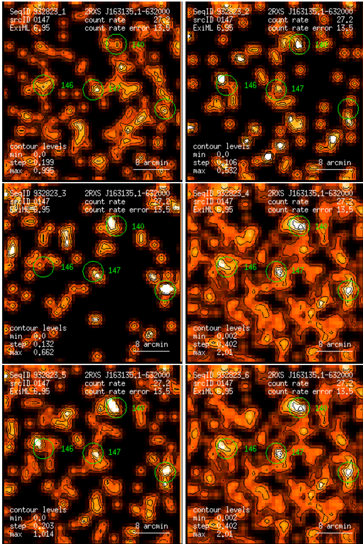
Figure 147: RASS 932823: detection 0147: band rate images, Gaussian filter: (1) PSPC channels 11 – 41, (2) 52 – 90, (3) 91 – 201, (4) 11 – 235, (5) 52 – 201, (6) 11 – 201. Broad band rates in counts/ks. Band rate contour levels in counts/ks/arcmin 2 .
