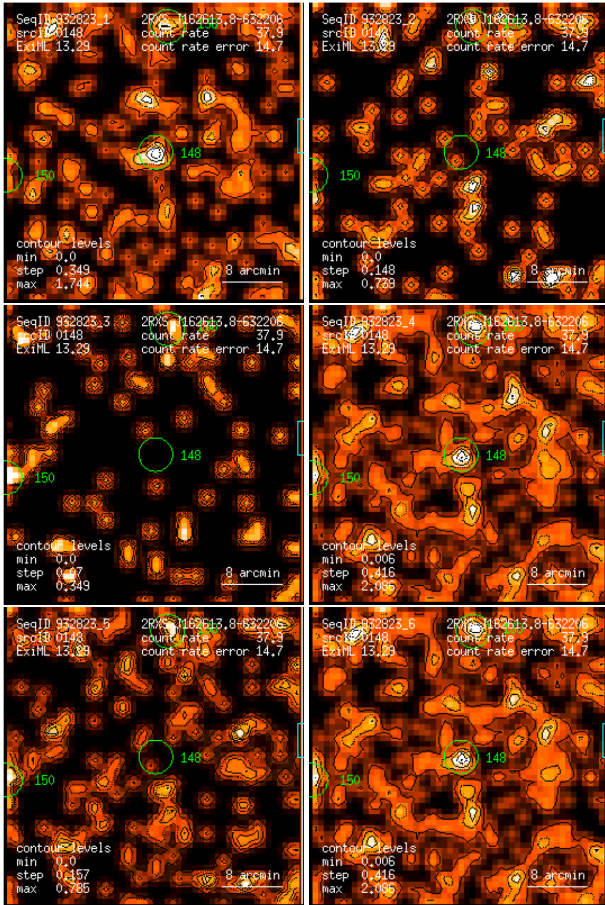
Figure 148: RASS 932823: detection 0148: band rate images, Gaussian filter: (1) PSPC channels 11 – 41, (2) 52 – 90, (3) 91 – 201, (4) 11 – 235, (5) 52 – 201, (6) 11 – 201. Broad band rates in counts/ks. Band rate contour levels in counts/ks/arcmin 2 .
