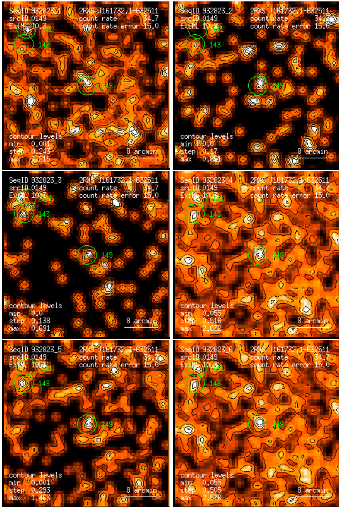
Figure 149: RASS 932823: detection 0149: band rate images, Gaussian filter: (1) PSPC channels 11 – 41, (2) 52 – 90, (3) 91 – 201, (4) 11 – 235, (5) 52 – 201, (6) 11 – 201. Broad band rates in counts/ks. Band rate contour levels in counts/ks/arcmin 2 .
