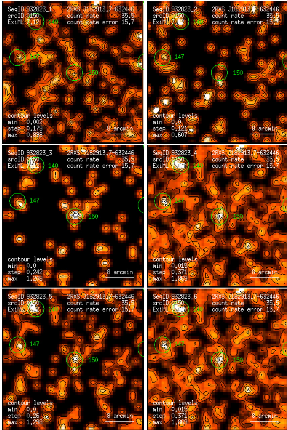
Figure 150: RASS 932823: detection 0150: band rate images, Gaussian filter: (1) PSPC channels 11 – 41, (2) 52 – 90, (3) 91 – 201, (4) 11 – 235, (5) 52 – 201, (6) 11 – 201. Broad band rates in counts/ks. Band rate contour levels in counts/ks/arcmin 2 .
