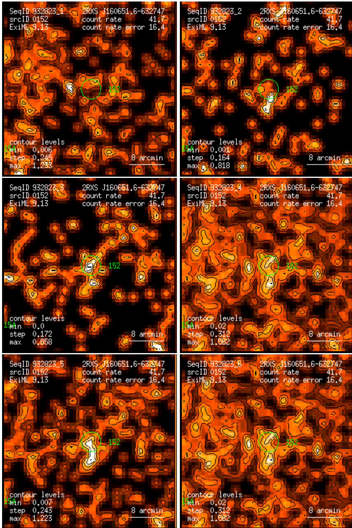
Figure 152: RASS 932823: detection 0152: band rate images, Gaussian filter: (1) PSPC channels 11 – 41, (2) 52 – 90, (3) 91 – 201, (4) 11 – 235, (5) 52 – 201, (6) 11 – 201. Broad band rates in counts/ks. Band rate contour levels in counts/ks/arcmin 2 .
