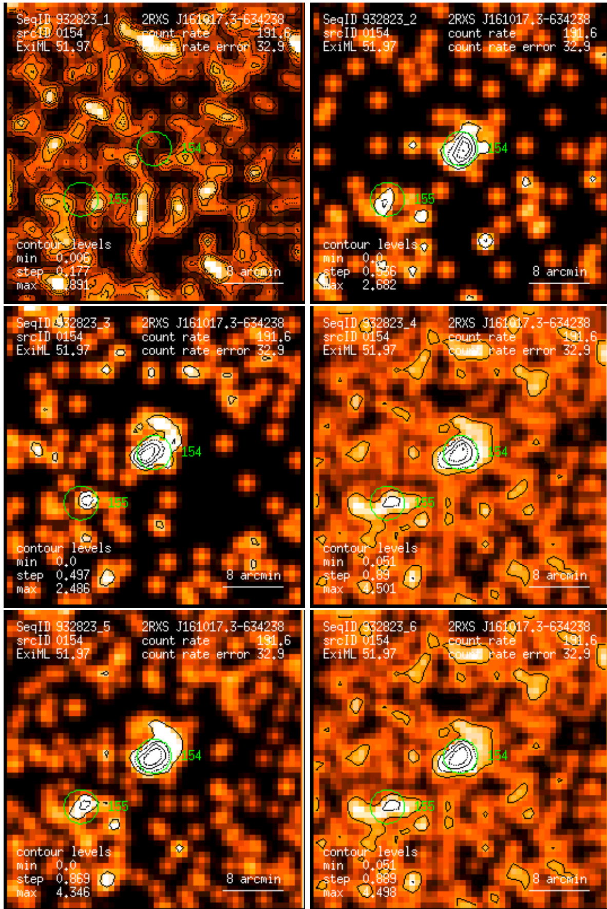
Figure 154: RASS 932823: detection 0154: band rate images, Gaussian filter: (1) PSPC channels 11 – 41, (2) 52 – 90, (3) 91 – 201, (4) 11 – 235, (5) 52 – 201, (6) 11 – 201. Broad band rates in counts/ks. Band rate contour levels in counts/ks/arcmin 2 .
