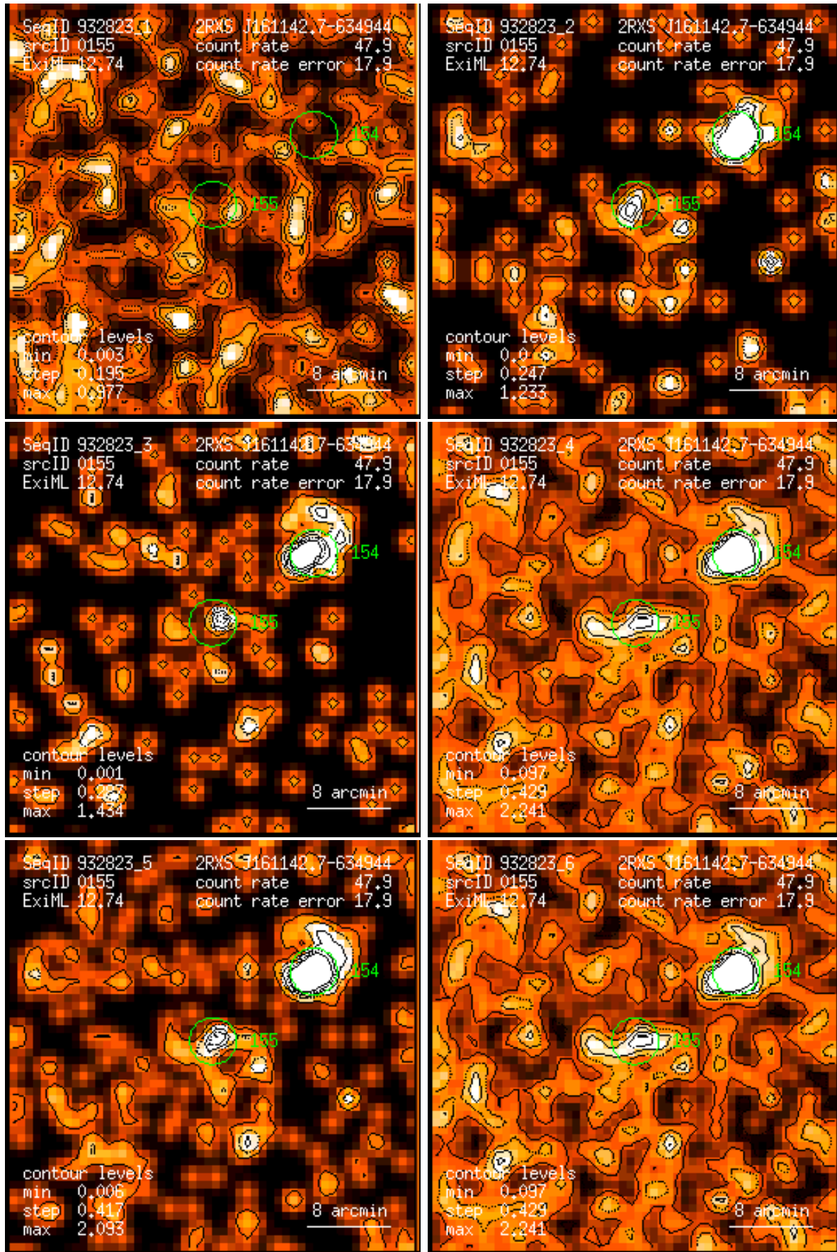
Figure 155: RASS 932823: detection 0155: band rate images, Gaussian filter: (1) PSPC channels 11 – 41, (2) 52 – 90, (3) 91 – 201, (4) 11 – 235, (5) 52 – 201, (6) 11 – 201. Broad band rates in counts/ks. Band rate contour levels in counts/ks/arcmin 2 .
