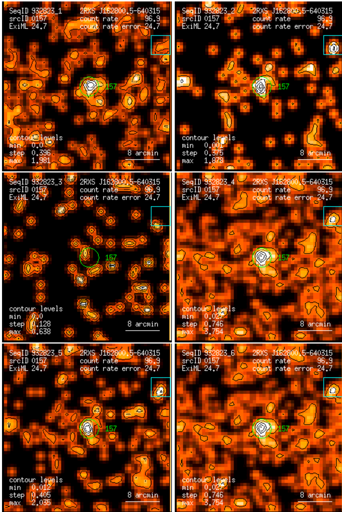
Figure 157: RASS 932823: detection 0157: band rate images, Gaussian filter: (1) PSPC channels 11 – 41, (2) 52 – 90, (3) 91 – 201, (4) 11 – 235, (5) 52 – 201, (6) 11 – 201. Broad band rates in counts/ks. Band rate contour levels in counts/ks/arcmin 2 .
