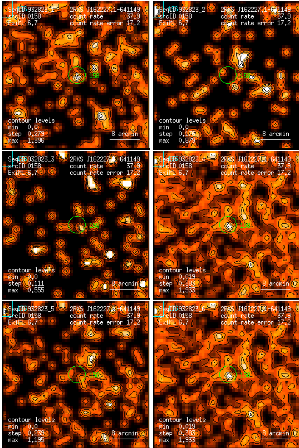
Figure 158: RASS 932823: detection 0158: band rate images, Gaussian filter: (1) PSPC channels 11 – 41, (2) 52 – 90, (3) 91 – 201, (4) 11 – 235, (5) 52 – 201, (6) 11 – 201. Broad band rates in counts/ks. Band rate contour levels in counts/ks/arcmin 2 .
