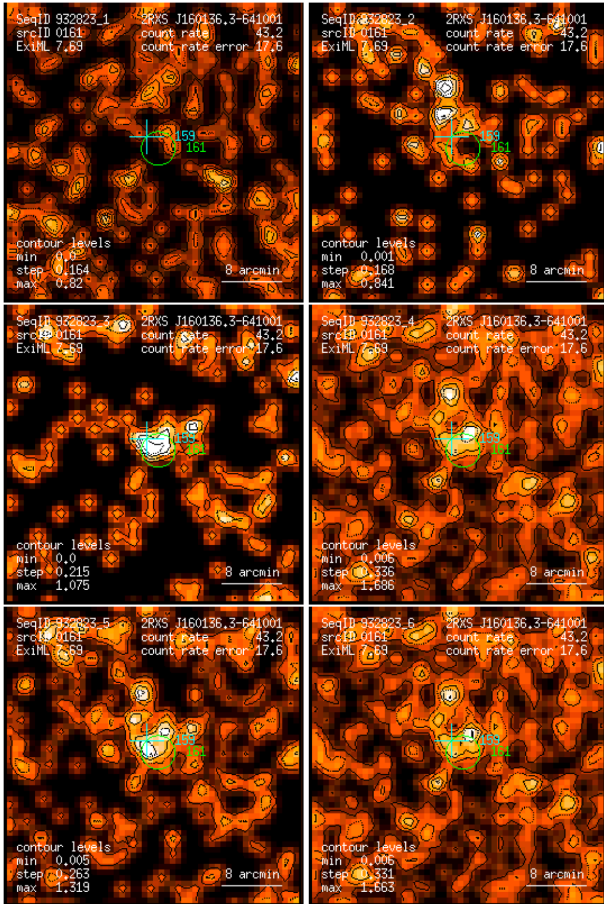
Figure 161: RASS 932823: detection 0161: band rate images, Gaussian filter: (1) PSPC channels 11 – 41, (2) 52 – 90, (3) 91 – 201, (4) 11 – 235, (5) 52 – 201, (6) 11 – 201. Broad band rates in counts/ks. Band rate contour levels in counts/ks/arcmin 2 .
