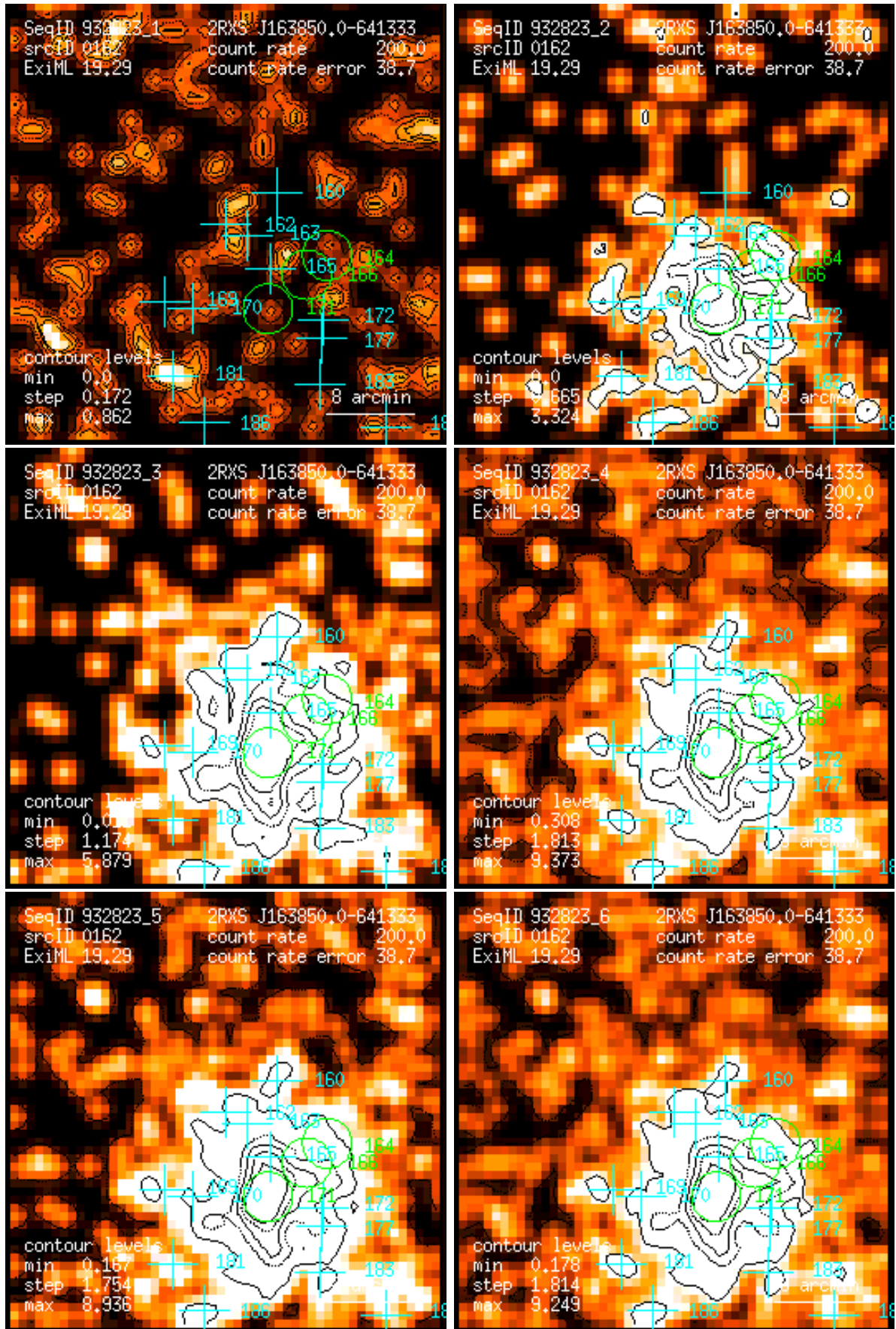
Figure 162: RASS 932823: detection 0162: band rate images, Gaussian filter: (1) PSPC channels 11 – 41, (2) 52 – 90, (3) 91 – 201, (4) 11 – 235, (5) 52 – 201, (6) 11 – 201. Broad band rates in counts/ks. Band rate contour levels in counts/ks/arcmin 2 .
