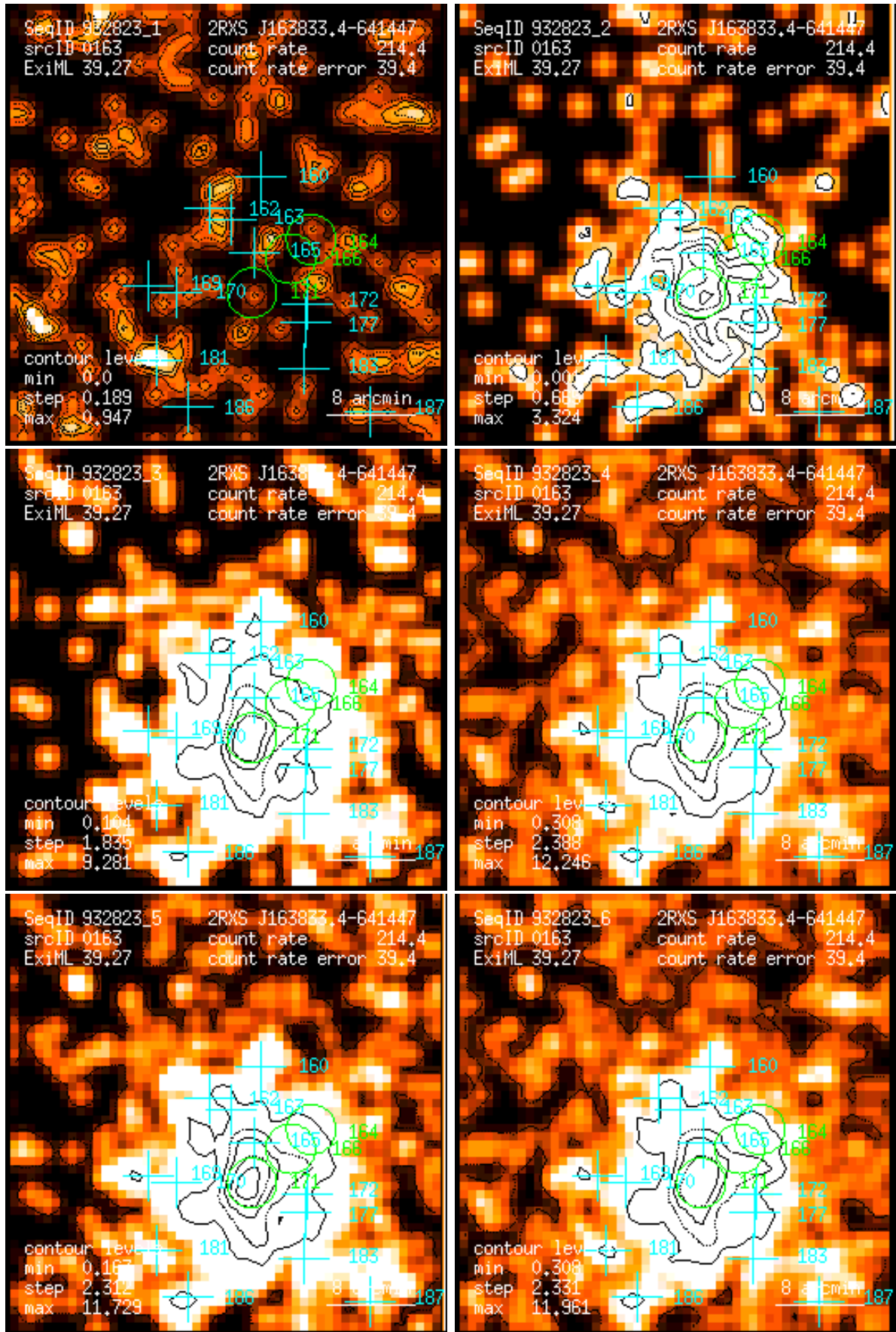
Figure 163: RASS 932823: detection 0163: band rate images, Gaussian filter: (1) PSPC channels 11 – 41, (2) 52 – 90, (3) 91 – 201, (4) 11 – 235, (5) 52 – 201, (6) 11 – 201. Broad band rates in counts/ks. Band rate contour levels in counts/ks/arcmin 2 .
