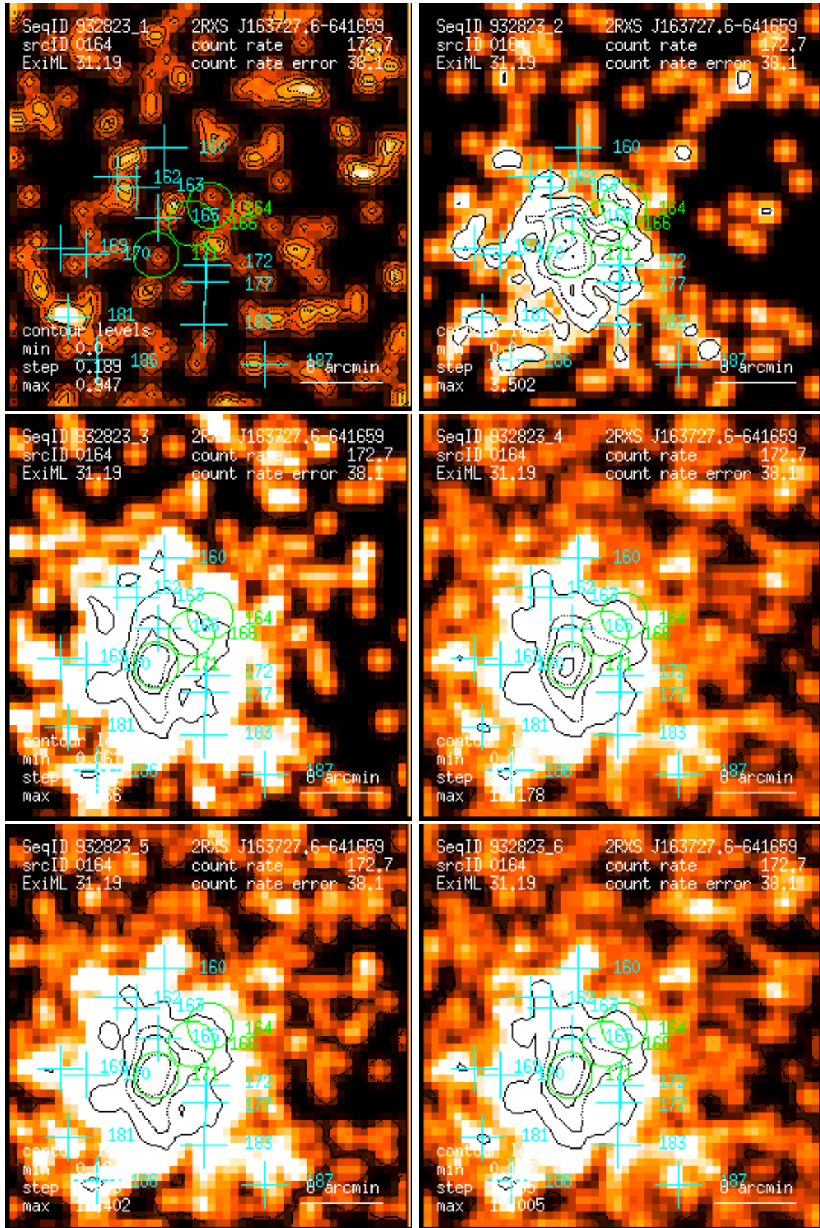
Figure 164: RASS 932823: detection 0164: band rate images, Gaussian filter: (1) PSPC channels 11 – 41, (2) 52 – 90, (3) 91 – 201, (4) 11 – 235, (5) 52 – 201, (6) 11 – 201. Broad band rates in counts/ks. Band rate contour levels in counts/ks/arcmin 2 .
