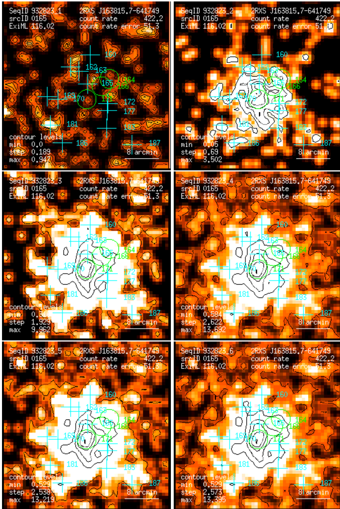
Figure 165: RASS 932823: detection 0165: band rate images, Gaussian filter: (1) PSPC channels 11 – 41, (2) 52 – 90, (3) 91 – 201, (4) 11 – 235, (5) 52 – 201, (6) 11 – 201. Broad band rates in counts/ks. Band rate contour levels in counts/ks/arcmin 2 .
