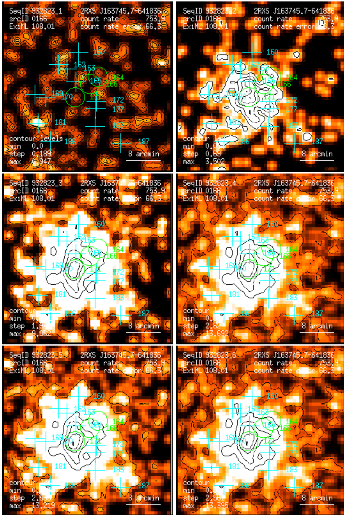
Figure 166: RASS 932823: detection 0166: band rate images, Gaussian filter: (1) PSPC channels 11 – 41, (2) 52 – 90, (3) 91 – 201, (4) 11 – 235, (5) 52 – 201, (6) 11 – 201. Broad band rates in counts/ks. Band rate contour levels in counts/ks/arcmin 2 .
