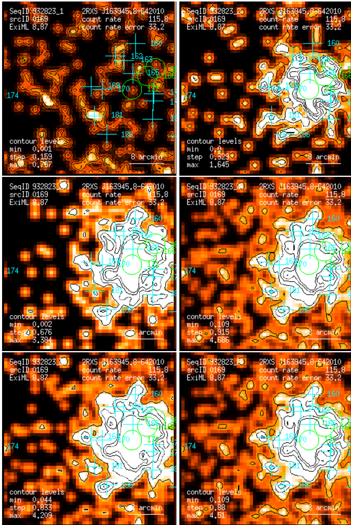
Figure 169: RASS 932823: detection 0169: band rate images, Gaussian filter: (1) PSPC channels 11 – 41, (2) 52 – 90, (3) 91 – 201, (4) 11 – 235, (5) 52 – 201, (6) 11 – 201. Broad band rates in counts/ks. Band rate contour levels in counts/ks/arcmin 2 .
