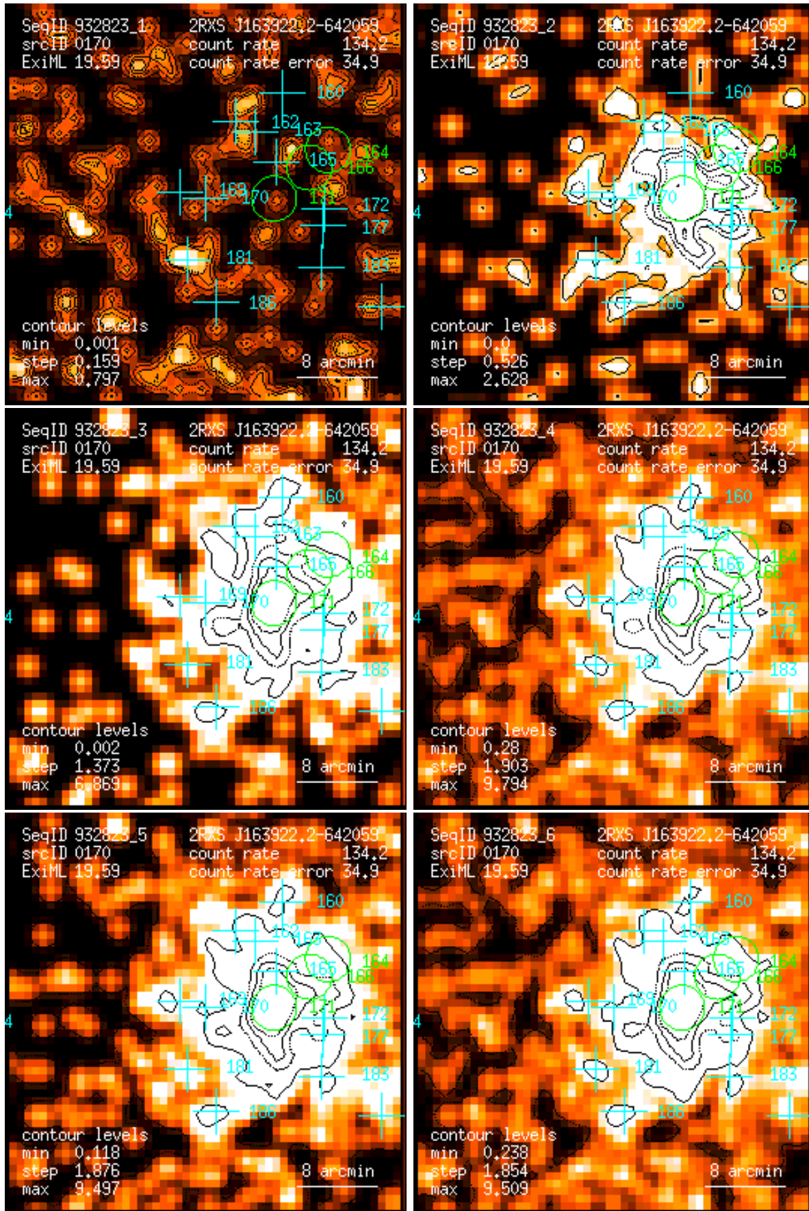
Figure 170: RASS 932823: detection 0170: band rate images, Gaussian filter: (1) PSPC channels 11 – 41, (2) 52 – 90, (3) 91 – 201, (4) 11 – 235, (5) 52 – 201, (6) 11 – 201. Broad band rates in counts/ks. Band rate contour levels in counts/ks/arcmin 2 .
