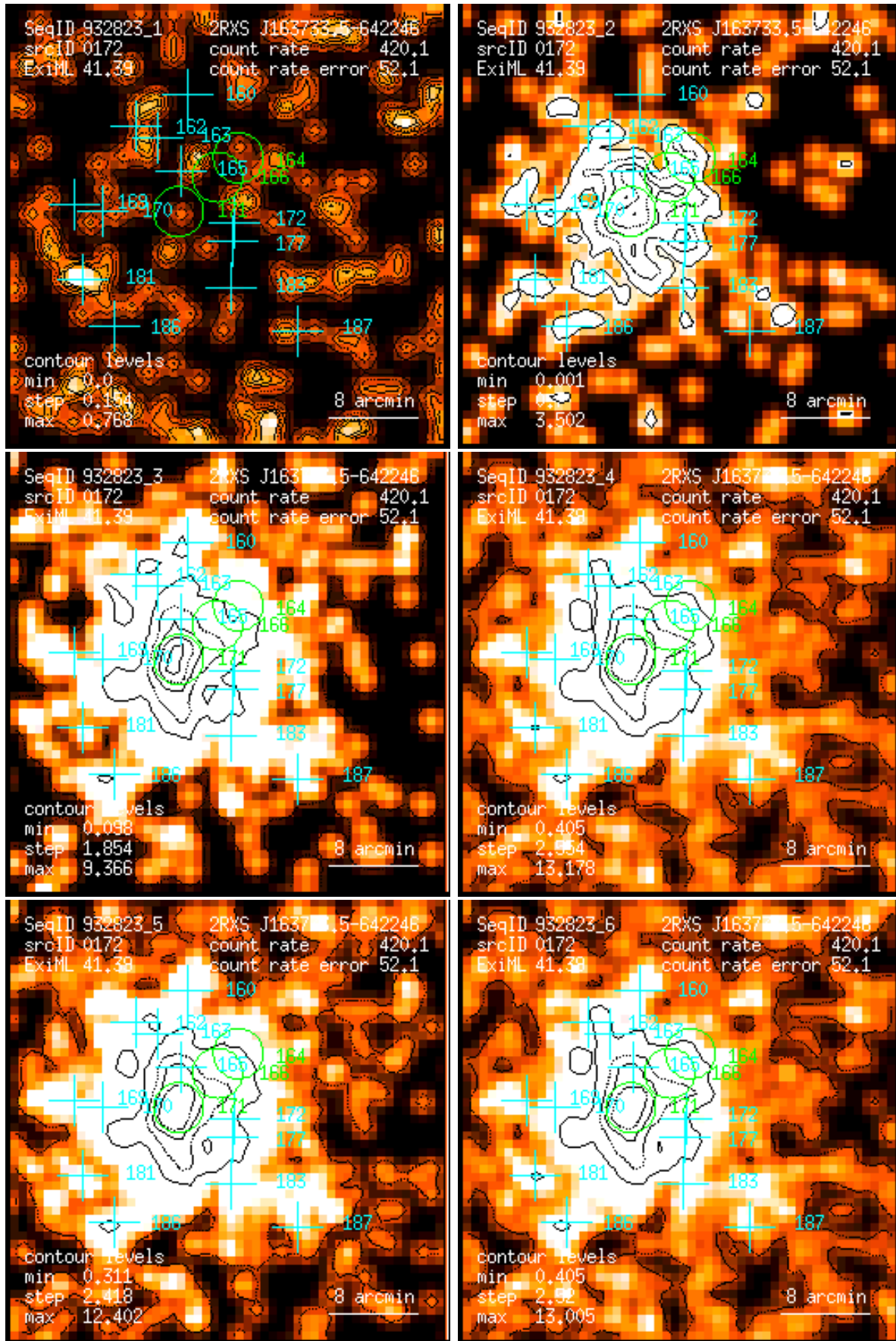
Figure 172: RASS 932823: detection 0172: band rate images, Gaussian filter: (1) PSPC channels 11 – 41, (2) 52 – 90, (3) 91 – 201, (4) 11 – 235, (5) 52 – 201, (6) 11 – 201. Broad band rates in counts/ks. Band rate contour levels in counts/ks/arcmin 2 .
