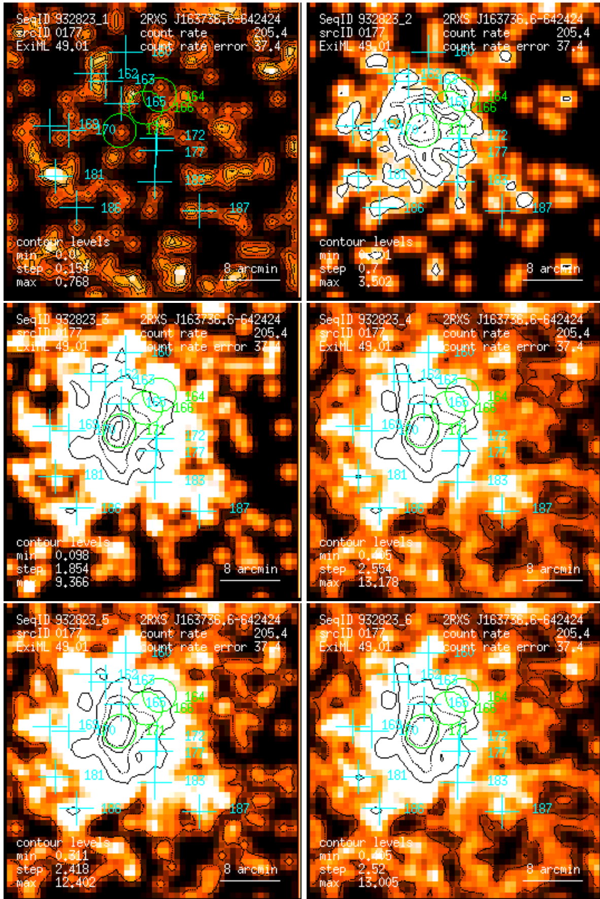
Figure 177: RASS 932823: detection 0177: band rate images, Gaussian filter: (1) PSPC channels 11 – 41, (2) 52 – 90, (3) 91 – 201, (4) 11 – 235, (5) 52 – 201, (6) 11 – 201. Broad band rates in counts/ks. Band rate contour levels in counts/ks/arcmin 2 .
