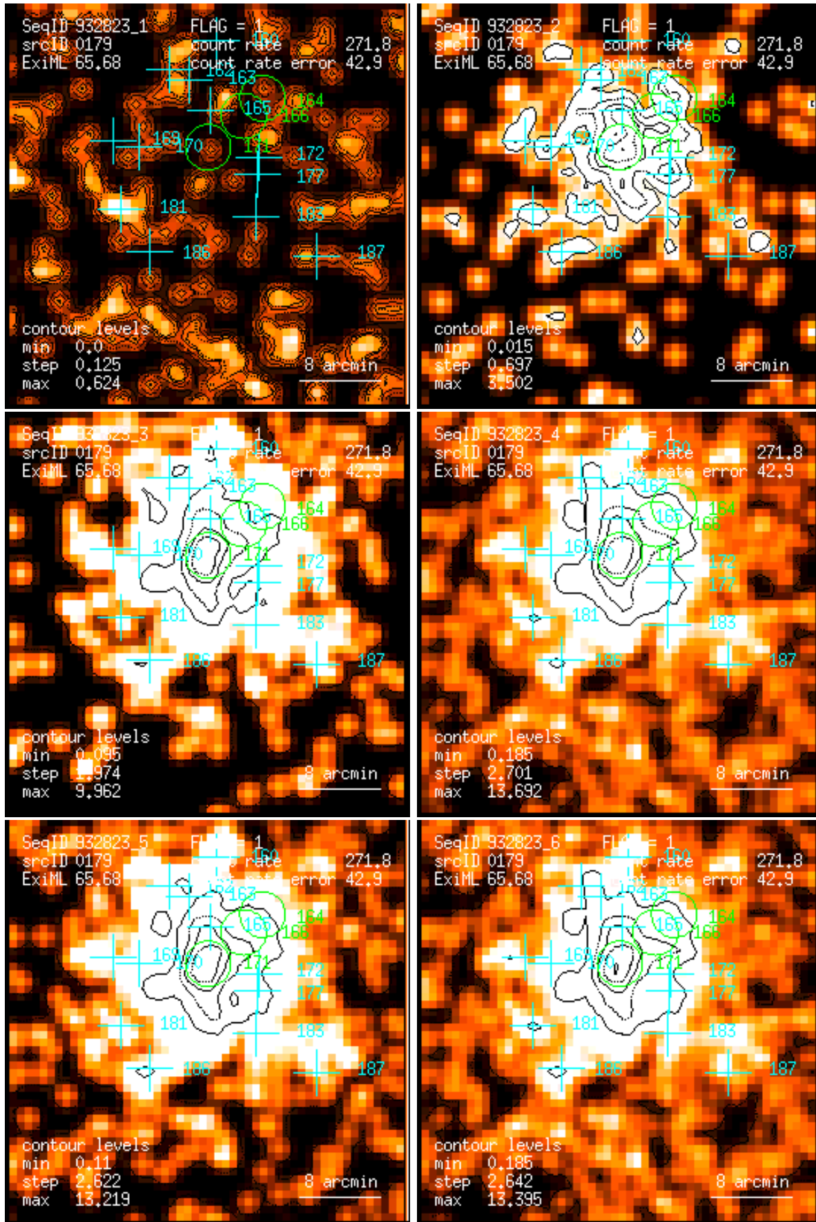
Figure 179: RASS 932823: detection 0179: band rate images, Gaussian filter: (1) PSPC channels 11 – 41, (2) 52 – 90, (3) 91 – 201, (4) 11 – 235, (5) 52 – 201, (6) 11 – 201. Broad band rates in counts/ks. Band rate contour levels in counts/ks/arcmin 2 .
