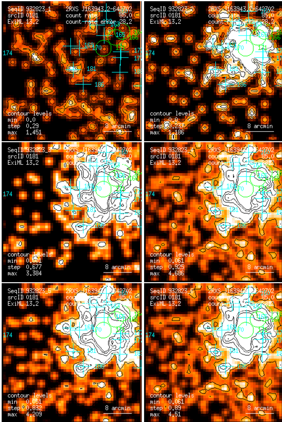
Figure 181: RASS 932823: detection 0181: band rate images, Gaussian filter: (1) PSPC channels 11 – 41, (2) 52 – 90, (3) 91 – 201, (4) 11 – 235, (5) 52 – 201, (6) 11 – 201. Broad band rates in counts/ks. Band rate contour levels in counts/ks/arcmin 2 .
