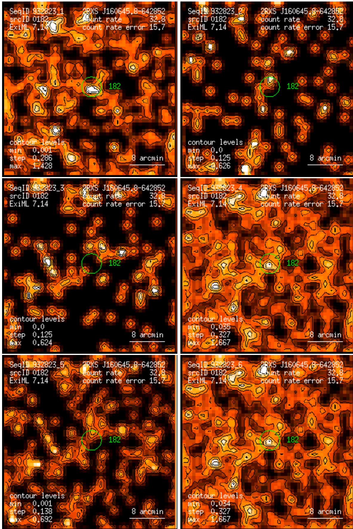
Figure 182: RASS 932823: detection 0182: band rate images, Gaussian filter: (1) PSPC channels 11 – 41, (2) 52 – 90, (3) 91 – 201, (4) 11 – 235, (5) 52 – 201, (6) 11 – 201. Broad band rates in counts/ks. Band rate contour levels in counts/ks/arcmin 2 .
