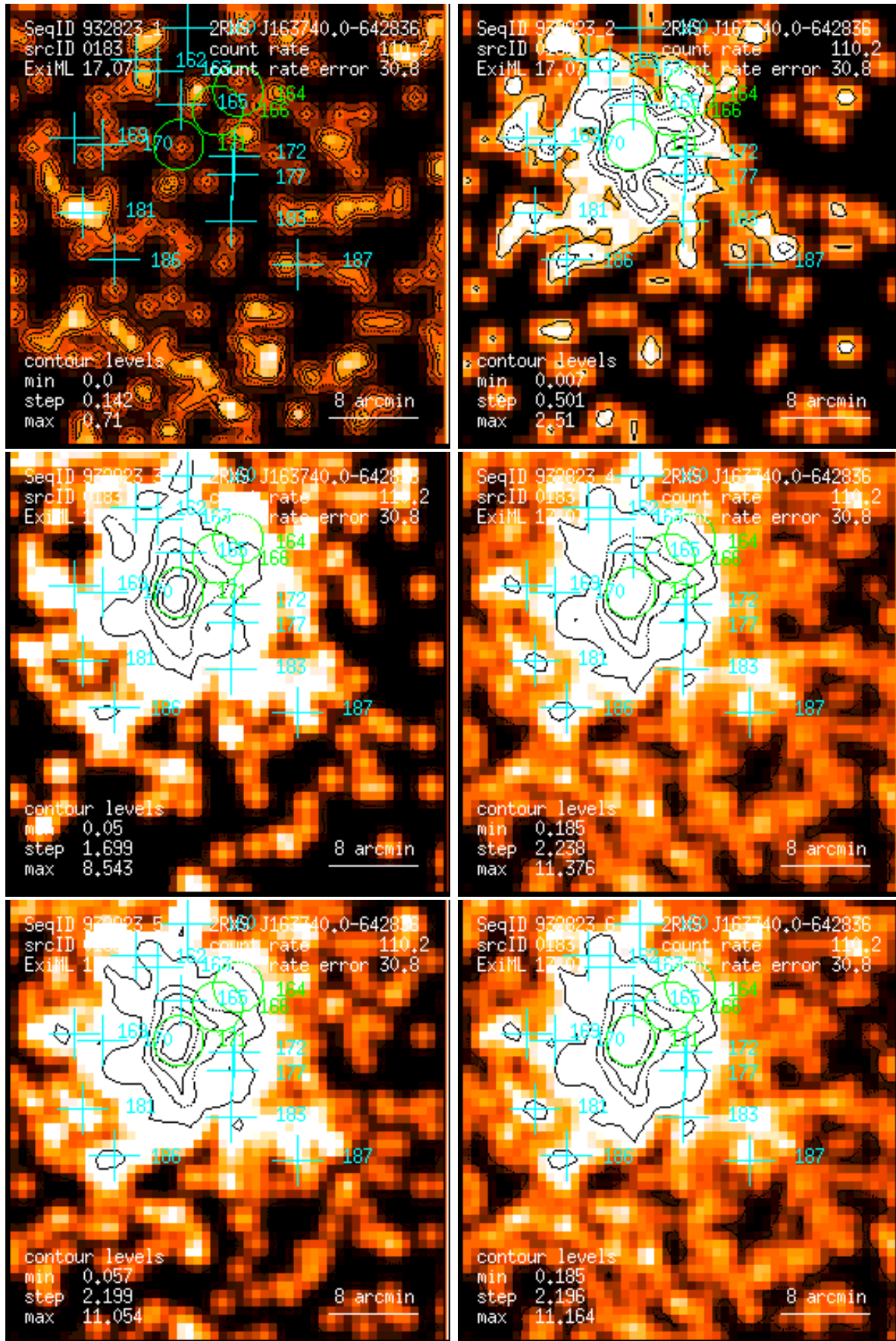
Figure 183: RASS 932823: detection 0183: band rate images, Gaussian filter: (1) PSPC channels 11 – 41, (2) 52 – 90, (3) 91 – 201, (4) 11 – 235, (5) 52 – 201, (6) 11 – 201. Broad band rates in counts/ks. Band rate contour levels in counts/ks/arcmin 2 .
