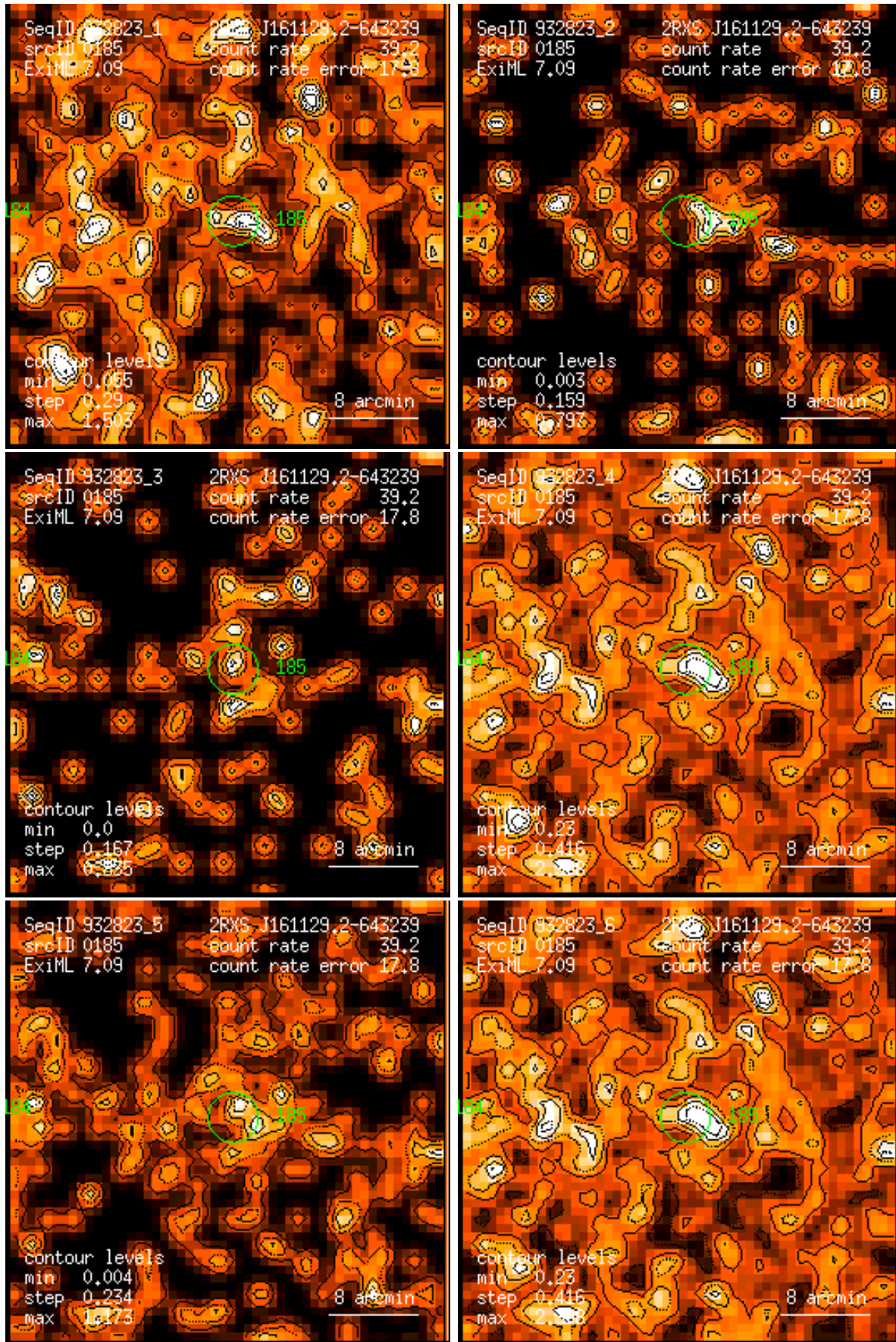
Figure 185: RASS 932823: detection 0185: band rate images, Gaussian filter: (1) PSPC channels 11 – 41, (2) 52 – 90, (3) 91 – 201, (4) 11 – 235, (5) 52 – 201, (6) 11 – 201. Broad band rates in counts/ks. Band rate contour levels in counts/ks/arcmin 2 .
