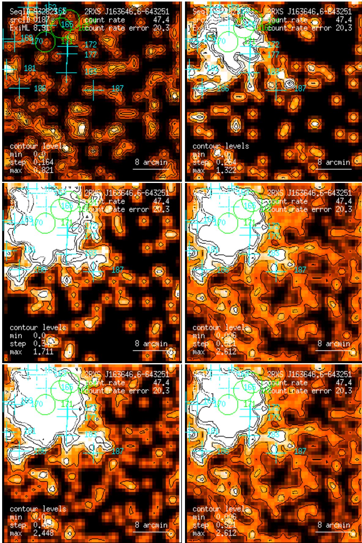
Figure 187: RASS 932823: detection 0187: band rate images, Gaussian filter: (1) PSPC channels 11 – 41, (2) 52 – 90, (3) 91 – 201, (4) 11 – 235, (5) 52 – 201, (6) 11 – 201. Broad band rates in counts/ks. Band rate contour levels in counts/ks/arcmin 2 .
