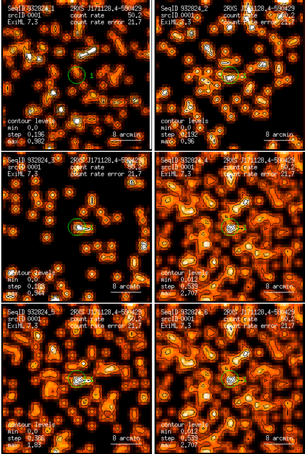
Figure 1: RASS 932824: detection 0001: band rate images, Gaussian filter: (1) PSPC channels 11 – 41, (2) 52 – 90, (3) 91 – 201, (4) 11 – 235, (5) 52 – 201, (6) 11 – 201. Broad band rates in counts/ks. Band rate contour levels in counts/ks/arcmin 2 .
