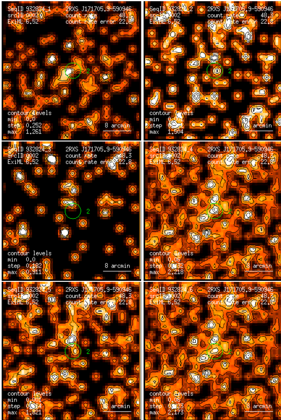
Figure 2: RASS 932824: detection 0002: band rate images, Gaussian filter: (1) PSPC channels 11 – 41, (2) 52 – 90, (3) 91 – 201, (4) 11 – 235, (5) 52 – 201, (6) 11 – 201. Broad band rates in counts/ks. Band rate contour levels in counts/ks/arcmin 2 .
