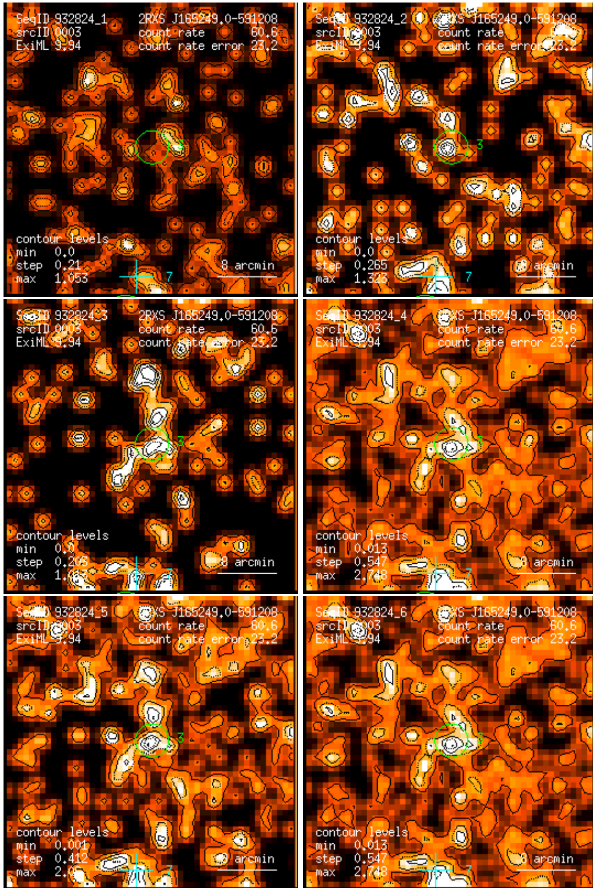
Figure 3: RASS 932824: detection 0003: band rate images, Gaussian filter: (1) PSPC channels 11 – 41, (2) 52 – 90, (3) 91 – 201, (4) 11 – 235, (5) 52 – 201, (6) 11 – 201. Broad band rates in counts/ks. Band rate contour levels in counts/ks/arcmin 2 .
