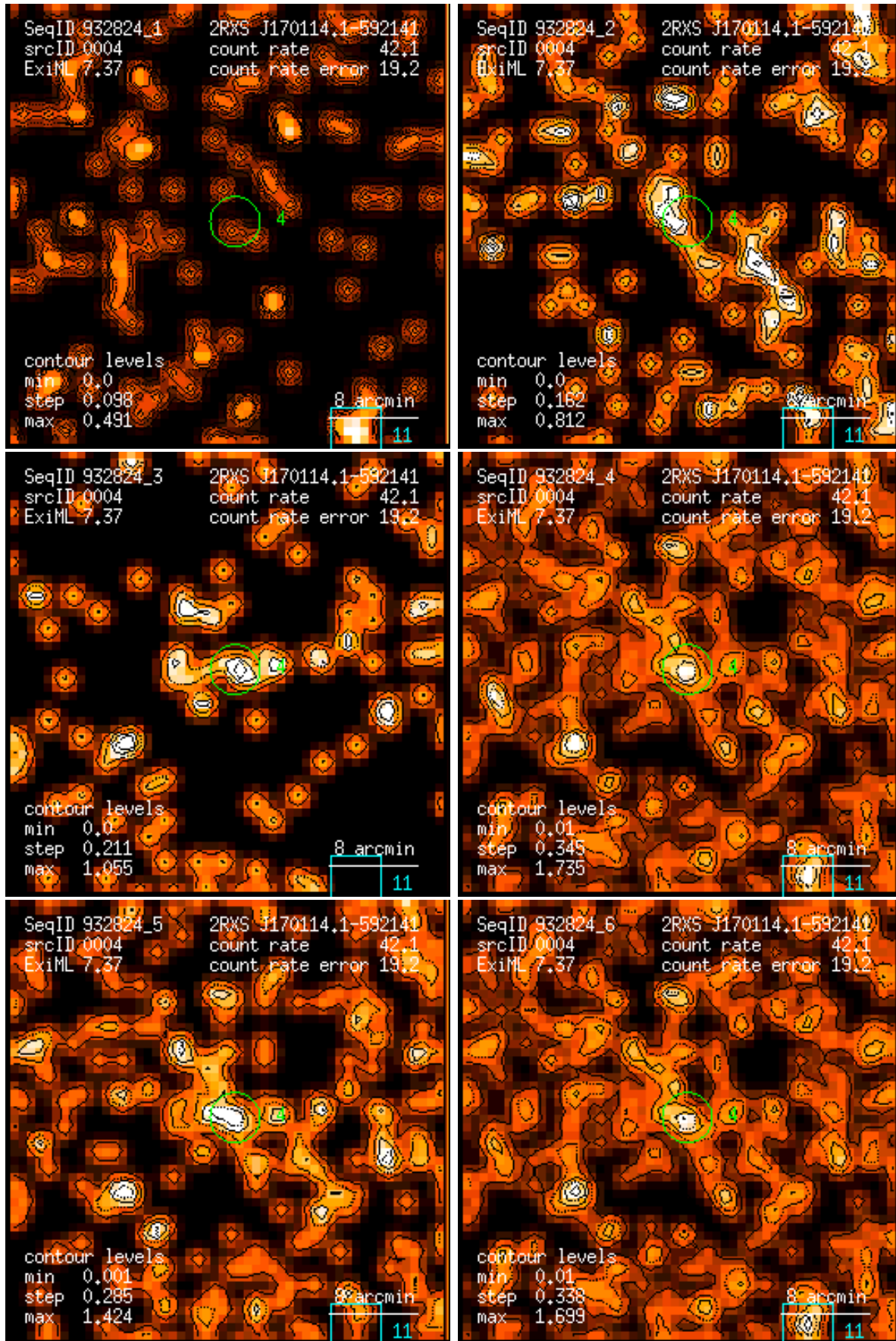
Figure 4: RASS 932824: detection 0004: band rate images, Gaussian filter: (1) PSPC channels 11 – 41, (2) 52 – 90, (3) 91 – 201, (4) 11 – 235, (5) 52 – 201, (6) 11 – 201. Broad band rates in counts/ks. Band rate contour levels in counts/ks/arcmin 2 .
