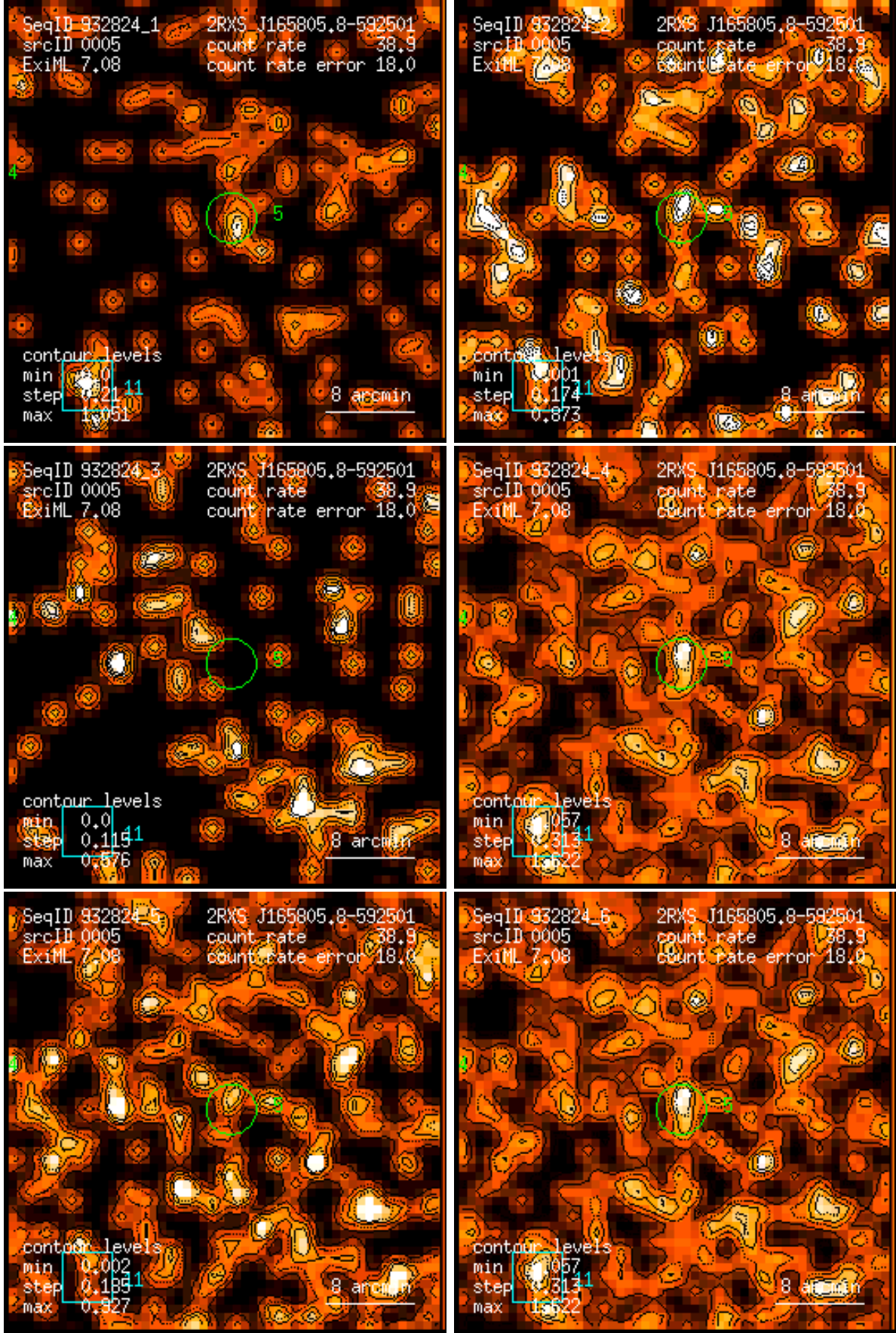
Figure 5: RASS 932824: detection 0005: band rate images, Gaussian filter: (1) PSPC channels 11 – 41, (2) 52 – 90, (3) 91 – 201, (4) 11 – 235, (5) 52 – 201, (6) 11 – 201. Broad band rates in counts/ks. Band rate contour levels in counts/ks/arcmin 2 .
