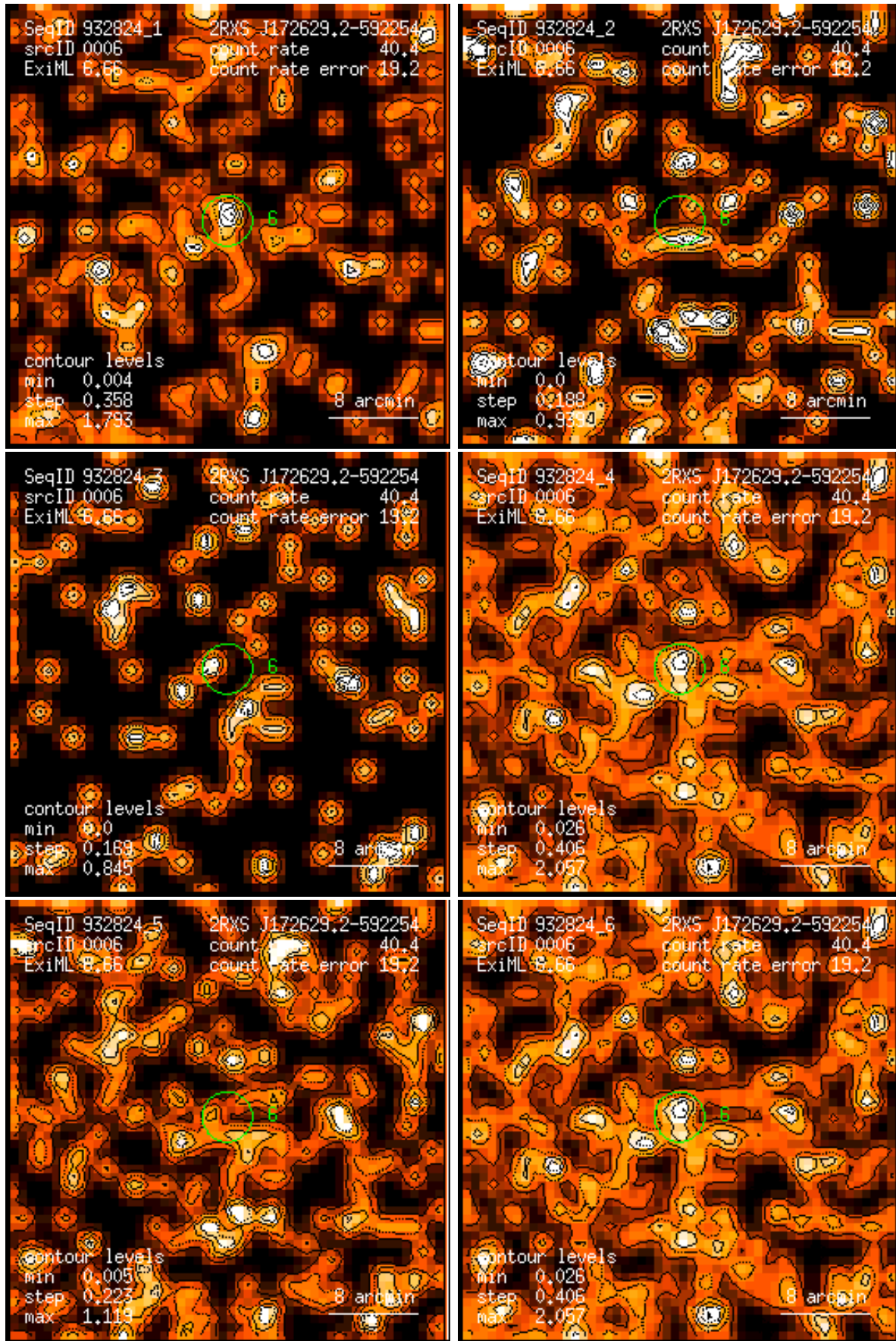
Figure 6: RASS 932824: detection 0006: band rate images, Gaussian filter: (1) PSPC channels 11 – 41, (2) 52 – 90, (3) 91 – 201, (4) 11 – 235, (5) 52 – 201, (6) 11 – 201. Broad band rates in counts/ks. Band rate contour levels in counts/ks/arcmin 2 .
