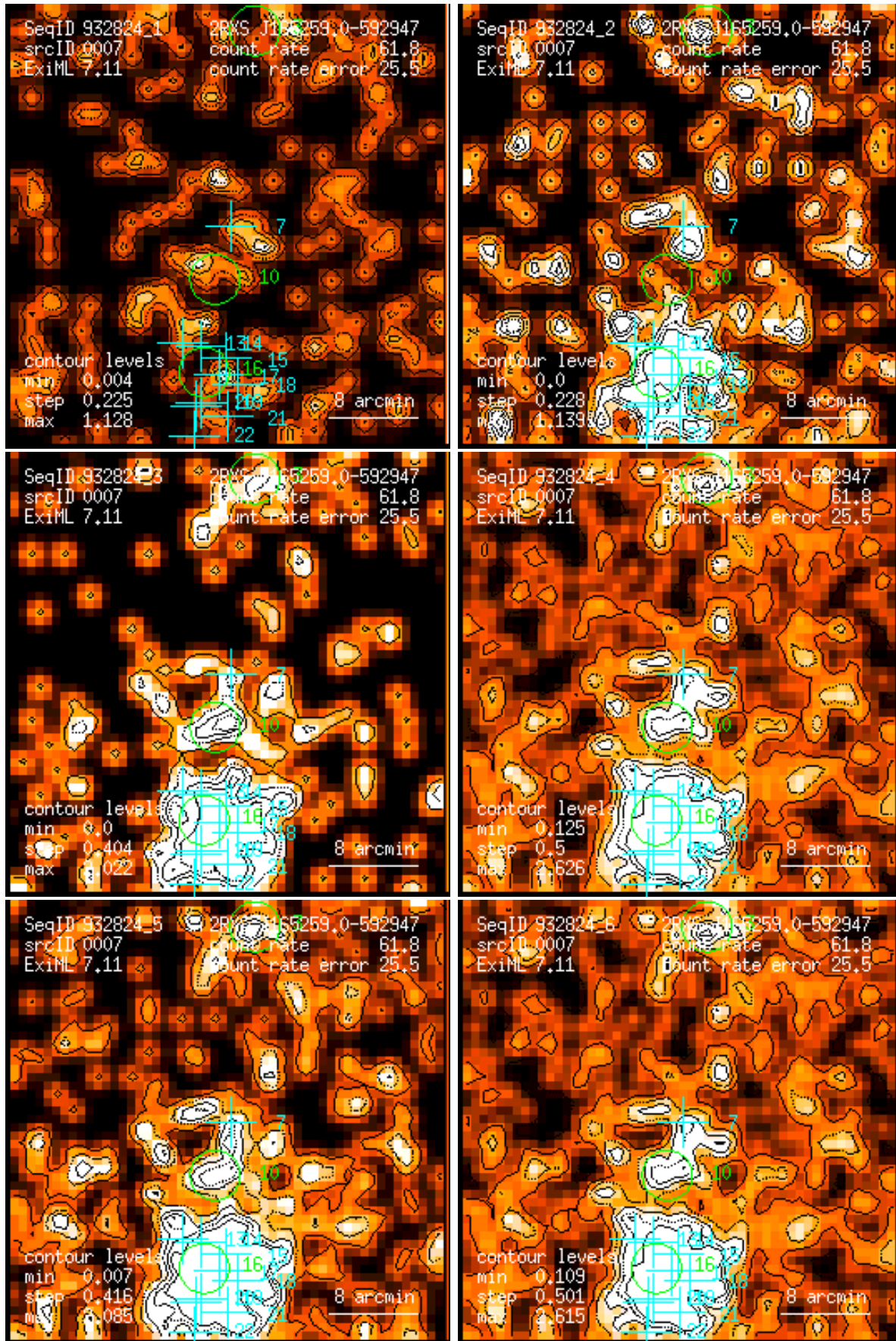
Figure 7: RASS 932824: detection 0007: band rate images, Gaussian filter: (1) PSPC channels 11 – 41, (2) 52 – 90, (3) 91 – 201, (4) 11 – 235, (5) 52 – 201, (6) 11 – 201. Broad band rates in counts/ks. Band rate contour levels in counts/ks/arcmin 2 .
