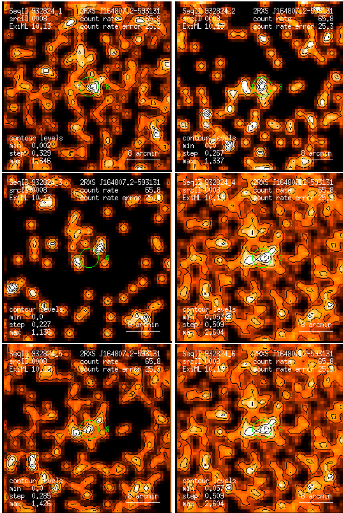
Figure 8: RASS 932824: detection 0008: band rate images, Gaussian filter: (1) PSPC channels 11 – 41, (2) 52 – 90, (3) 91 – 201, (4) 11 – 235, (5) 52 – 201, (6) 11 – 201. Broad band rates in counts/ks. Band rate contour levels in counts/ks/arcmin 2 .
