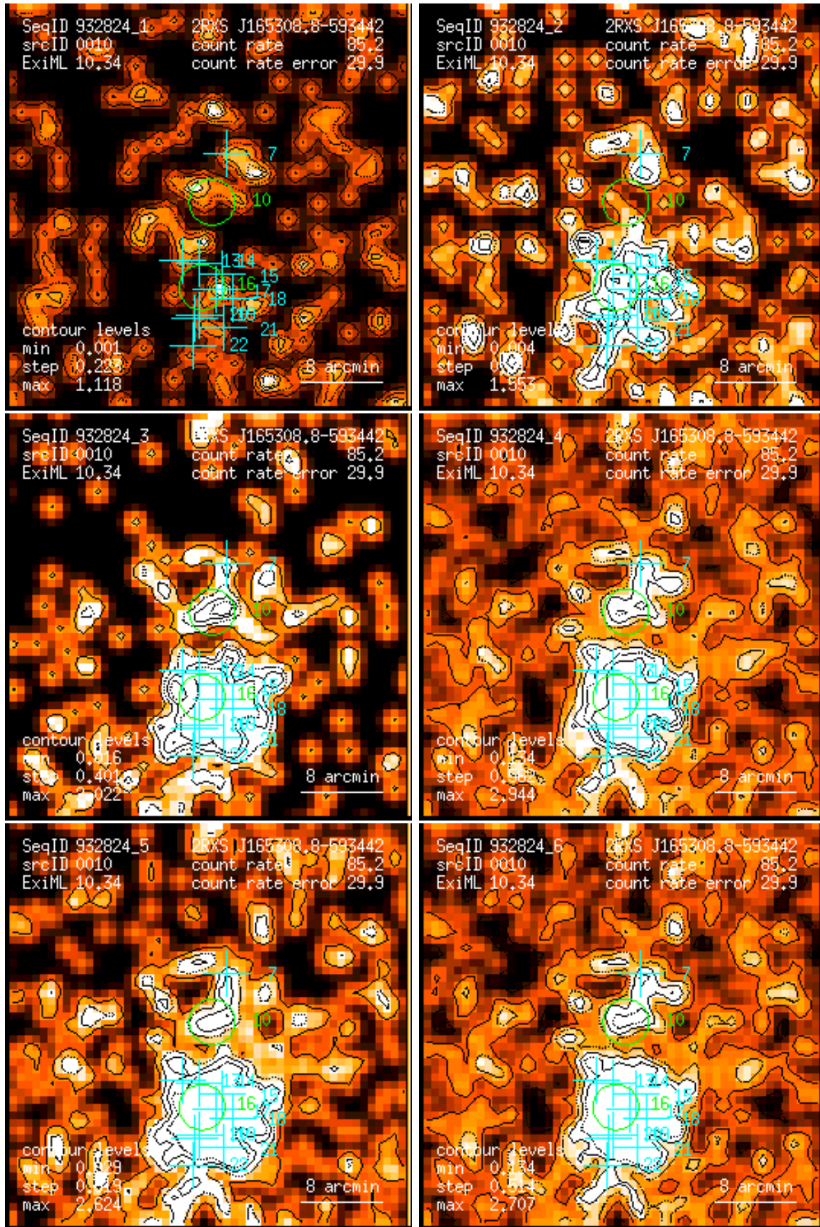
Figure 10: RASS 932824: detection 0010: band rate images, Gaussian filter: (1) PSPC channels 11 – 41, (2) 52 – 90, (3) 91 – 201, (4) 11 – 235, (5) 52 – 201, (6) 11 – 201. Broad band rates in counts/ks. Band rate contour levels in counts/ks/arcmin 2 .
