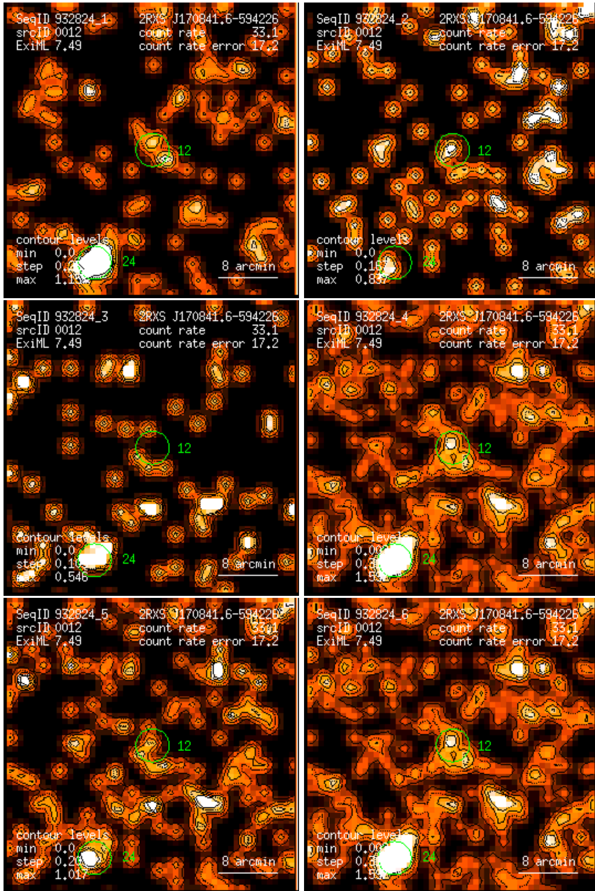
Figure 12: RASS 932824: detection 0012: band rate images, Gaussian filter: (1) PSPC channels 11 – 41, (2) 52 – 90, (3) 91 – 201, (4) 11 – 235, (5) 52 – 201, (6) 11 – 201. Broad band rates in counts/ks. Band rate contour levels in counts/ks/arcmin 2 .
