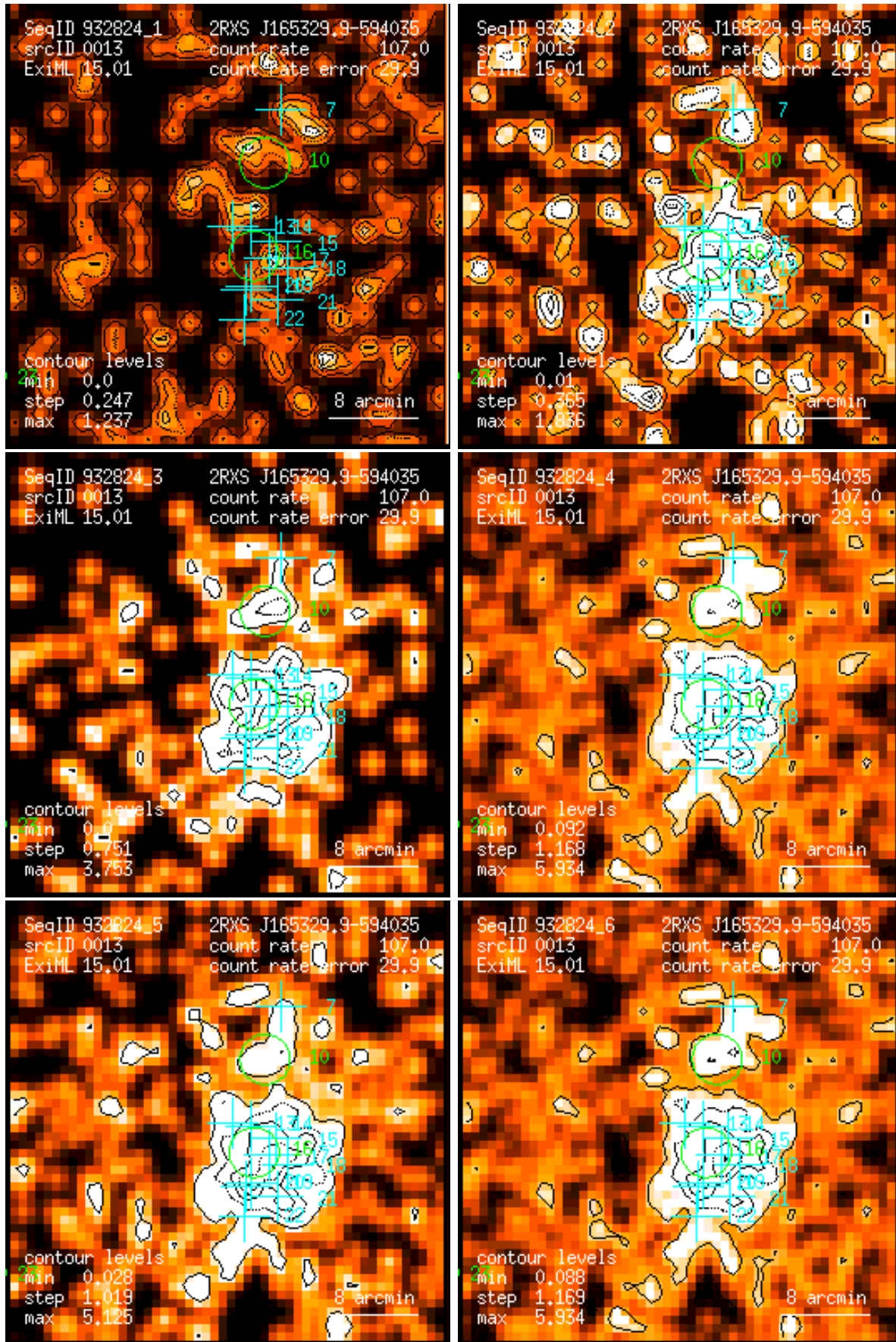
Figure 13: RASS 932824: detection 0013: band rate images, Gaussian filter: (1) PSPC channels 11 – 41, (2) 52 – 90, (3) 91 – 201, (4) 11 – 235, (5) 52 – 201, (6) 11 – 201. Broad band rates in counts/ks. Band rate contour levels in counts/ks/arcmin 2 .
